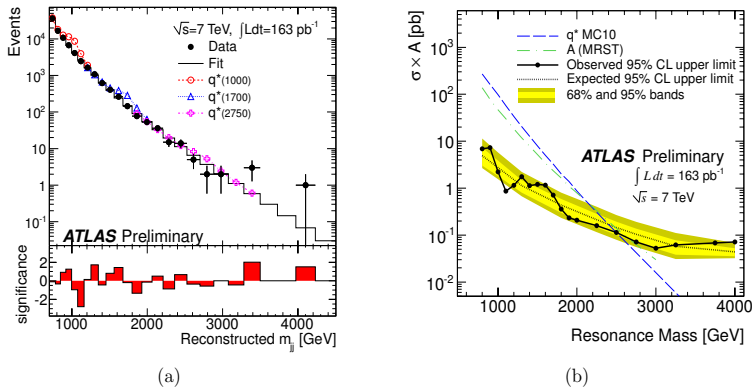
Figure 2: (a) Data dijet mass distribution (filled points) with background fit described by Eqn. 3 (histogram). q^* signals for excited-quark masses of 1, 1.7 and 2.75 TeV are plotted on top of the background.
