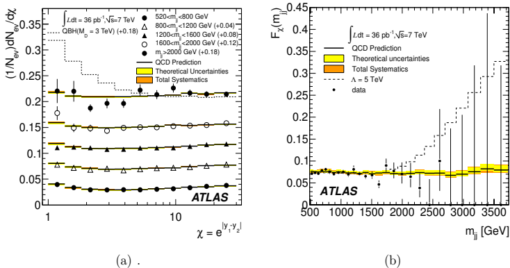
Figure 1: (a) The \chi distributions for 520 < m_{jj} < 800 GeV, 800 < m_{jj} < 1200 GeV, 1200 < m_{jj} < 1600 GeV, 1600 < m_{jj} < 2000 GeV and m_{jj} > 2000 GeV and (b) F_\chi(m_{jj}) distribution versus m_{jj} . Shown are the QCD predictions with systematics uncertainties (narrow bands), and data points with statistical uncertainties. Note that in (a) the distributions and QCD predictions have been offset by the amount shown in the legend to aid in visually comparing the shapes in each mass bin.
