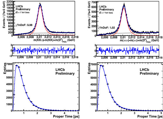
Figure 1: Top row: fits to the difference between the D^* and D^0 masses for a subset of the data, where the D^0 decays into K^+K^- (left) and \pi^+\pi^- (right). Bottom row: fits to the D^0 \rightarrow K^+K^- (left) and \bar{D}^0 \rightarrow K^+K^- (right) lifetime. The fit results are 407.6 \pm 2.4 and 409.2 \pm 2.4 fs respectively (statistical errors only).
