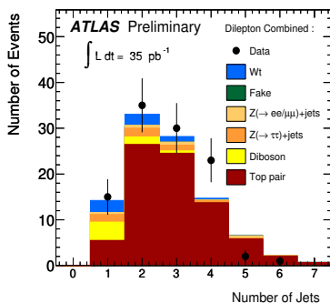
Figure 3: Jet-multiplicity for the single top Wt dilepton analysis.
