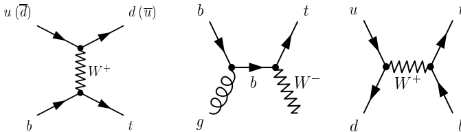
Figure 1: Feynman diagrams for single top quark production in the t -channel, Wt associated production and s -channel mode.
