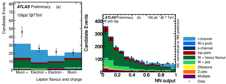
Figure 2: (a) Single top t -channel cut-based events separated by lepton flavour and charge and (b) neural network output distribution.
