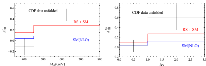
Figure 1: Left : The full top quark asymmetry integrated in the two energy ranges [350, 450] and [450, 900] of invariant mass M_{t\bar{t}} (in GeV) computed within the RS extension of the SM, A_{FB}^t , with \mu_F = \mu_R = m_t = 172.5 GeV [red lines] and compared to the SM prediction at NLO, A_{FB}^{SM} [blue lines] as well as to the unfolded CDF data for m_t = 172.5 GeV [black crosses for experimental errors]. Right : The asymmetries A_{FB}^{|\Delta y| < 1} and A_{FB}^{|\Delta y| > 1} computed in the RS extension [red lines] and compared to the SM prediction at NLO [blue lines] as well as to the unfolded CDF data [black crosses].
