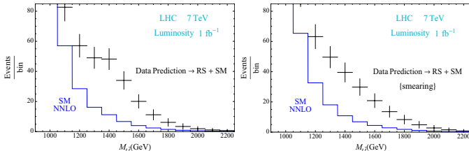
Figure 2: The distributions of the invariant mass M_{t\bar{t}} (in GeV) at the LHC assuming 100 GeV bins with a luminosity of \mathcal{L} = 1 \text{ fb}^{-1} . The SM at approximate NNLO ( \mu_F = \mu_R = m_t = 173 \text{ GeV} ) [blue histogram] is shown together with the RS contribution [in black]. The effect of smearing is only implemented in the right-hand side figure.
