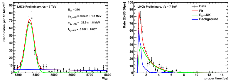
Figure 1: Left: Fit to the B_s^0 \rightarrow K^+ K^- mass spectrum with a Gaussian model of the signal and a first degree polynomial of the combinatorial background. Right: Fit to the total time distribution with the components of the signal and background shown in the plot. Both plots are for the absolute lifetime measurement.
