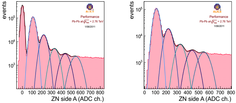
Figure 2: ZNA ADC spectra requiring signal in ZNA or ZNC (left) or in ZNA but not in ZNC (right).
