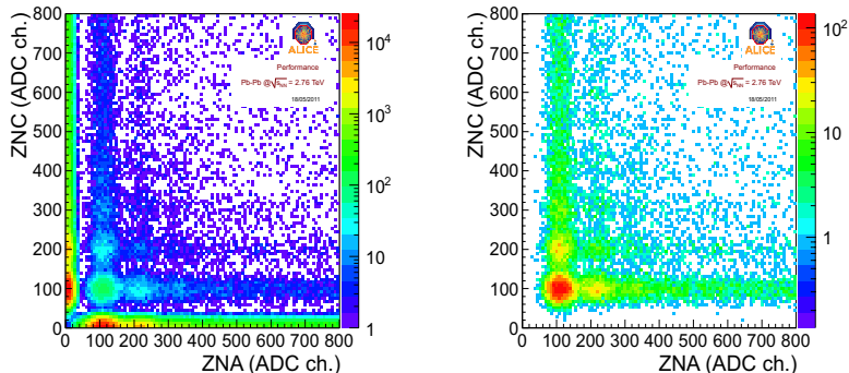
Figure 1: ZNC vs. ZNA ADC signal for single EMD plus hadronic events (left) and for mutual EMD plus hadronic events (right). The 1n signal is at channel \sim 100 .
