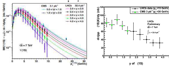
Figure 2: Left: Double differential \Upsilon(1S) cross section as a function of \Upsilon(1S)p_T , as measured by the CMS and LHCb experiments. Right: \Upsilon(1S) cross section integrated over p_T as a function of y for the CMS and LHCb experiments.
