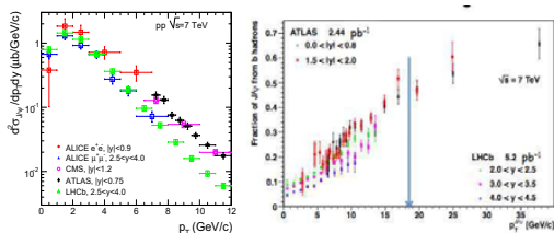
Figure 1: Left: Inclusive J/\psi cross section as a function of J/\psi p_T for the four LHC experiments. Right: Fraction of J/\psi from B as a function of J/\psi p_T measured by ATLAS and LHCb.
