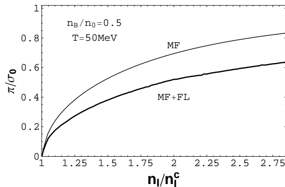
FIG. 1: The pion condensates in mean field approximation (thin line) and including meson fluctuations (thick line) as functions of isospin density at fixed temperature and baryon density. \sigma_0 is the chiral condensate in vacuum and n_I^c is the critical isospin density of pion superfluidity.
