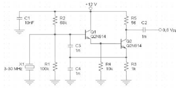
Figure 1: Colpitts oscillator from 3 to 30 MHz.
