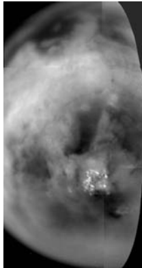
Figure 10: Image of the Titan’s south polar region acquired by the Image Science Subsystem, ISS, on board the Cassini spacecraft with filters designed to see through the thick haze and atmosphere [57]. The bright spots near the bottom represent a field of clouds near the south pole. There are many strange dark and bright patterns on Titan’s surface – linear, sinuous and circular. The smallest features detected on the surface are about 10 kilometers.
