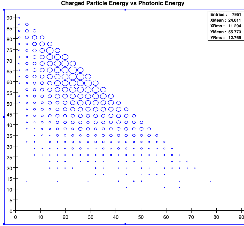
Figure 2: Total charged particle energy (GeV) vs total photon energy (GeV) for hadronic Z events with no neutrinos.
