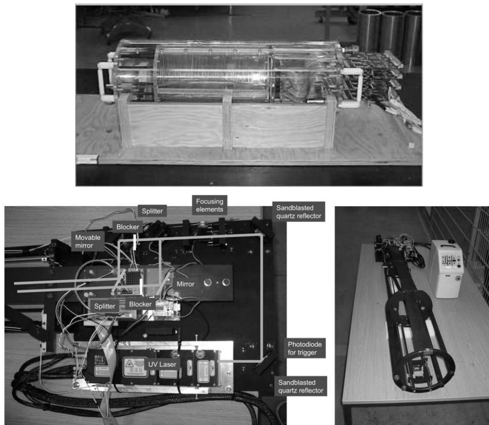
Figure 1: The upper photograph shows the prototype TPC, with the STAR front end cards connected on the right. The lower figures show the laser delivery system including the holding bracket for the TPC and the laser power supply.
