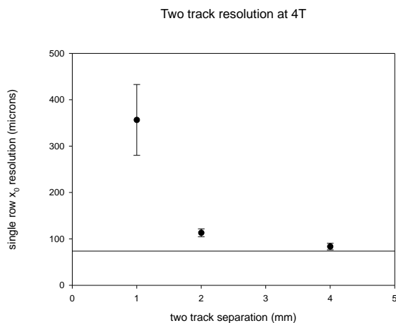
Figure 3: The degradation in transverse resolution is shown as a function of transverse separation between two parallel laser tracks. This is shown for P5 data at 4T.
