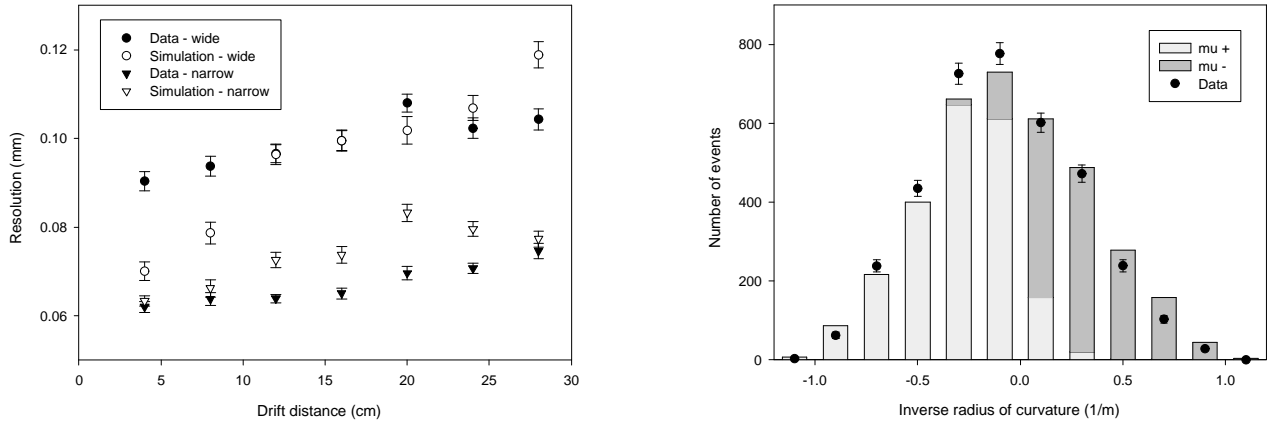
Figure 5: On the left, the measured resolution for wide and narrow pad cosmic data is shown, and compared to simulation results. On the right, the signed inverse radius of curvature is shown for the wide pad data, compared to the expected distributions separately shown for positive and negative cosmic muons.
