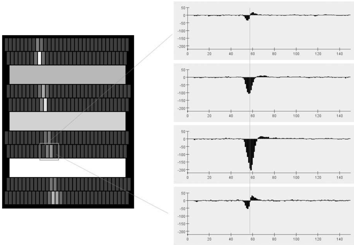
Figure 2: A typical cosmic ray track observed with the wide pad layout at 4T with P5 gas. The brightness of the pads indicates the amount of charged collected. The wide pads are used during data taking for selecting events that contain a track in the active area. The pulses for 4 neighbouring pads are shown on the right.
