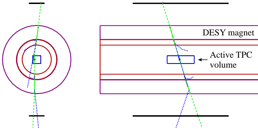
Figure 4: Example event from the GEANT3 simulation of cosmic events.
