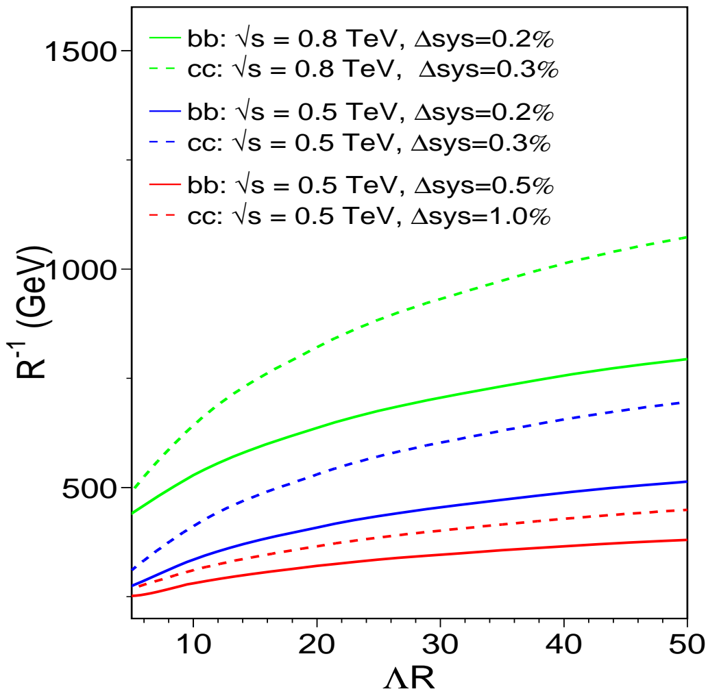
Figure 2: Limits at 95% C.L. on 1/R derived from measurements of b\bar{b} or c\bar{c} final states assuming different systematic errors. Deviations from the SM expectations can be observed up to the given values.
