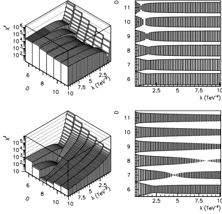
Figure 2: Upper part: values of the \chi^2/d.o.f. for the reconstructed spectra as a function of D and \lambda for "input" values \lambda = 1 \text{ TeV}^{-2} and D = 10 ; the right side shows rectangles proportional to the logarithm of the \chi^2/d.o.f. Lower part (left and right): values of the \chi^2/d.o.f. for the reconstructed spectra as a function of D and \lambda for "input" values \lambda = 5 \text{ TeV}^{-2} and D = 8 ; the right side shows rectangles proportional to the logarithm of the \chi^2/d.o.f.
