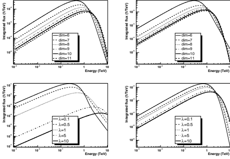
Figure 1: Integrated flux as a function of the total energy of the emitted quanta for an initial black hole mass M = 10 TeV. Upper left: \lambda = 0 , D = 6, 7, 8, 9, 10, 11 . Upper right: \lambda = 0, 5 TeV ^{-2} , D = 6, 7, 8, 9, 10, 11 . Lower left: D = 6 , \lambda = 0.1, 0.5, 1, 5, 10 TeV ^{-2} . Lower right: D = 11 , \lambda = 0.1, 0.5, 1, 5, 10 TeV ^{-2} .
