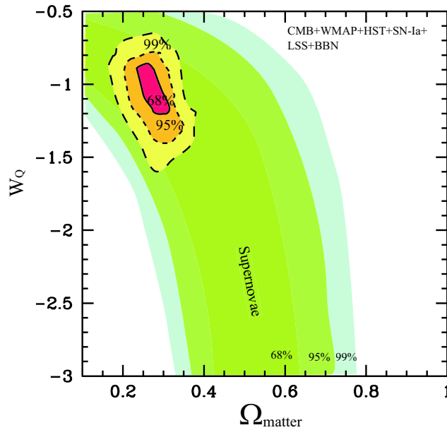
Figure 3: Limits on the equation-of-state parameter w in a flat universe, where \Omega_M + \Omega_X = 1 . From Melchiorri, Mersini, Ödman & Trodden 2003.
