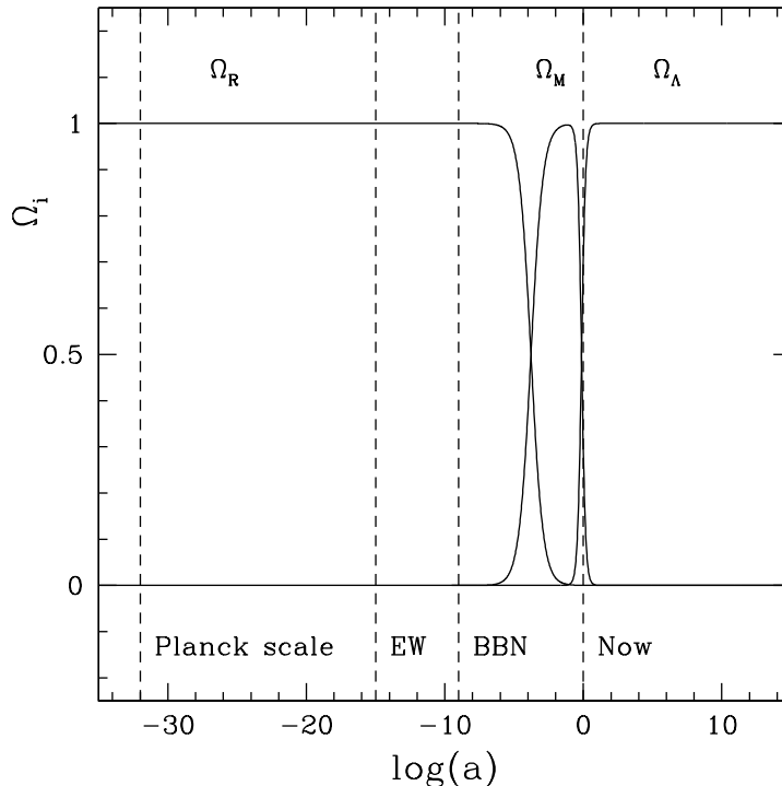
Figure 1: Density parameters \Omega_i for radiation (R), matter (M), and vacuum ( \Lambda ), as a function of the scale factor a , in a universe with \Omega_{\Lambda 0} = 0.7 , \Omega_{M0} = 0.3 , \Omega_{R0} = 5 \times 10^{-5} . Scale factors corresponding to the Planck era, electroweak symmetry breaking (EW), and Big Bang nucleosynthesis (BBN) are indicated, as well as the present day.
