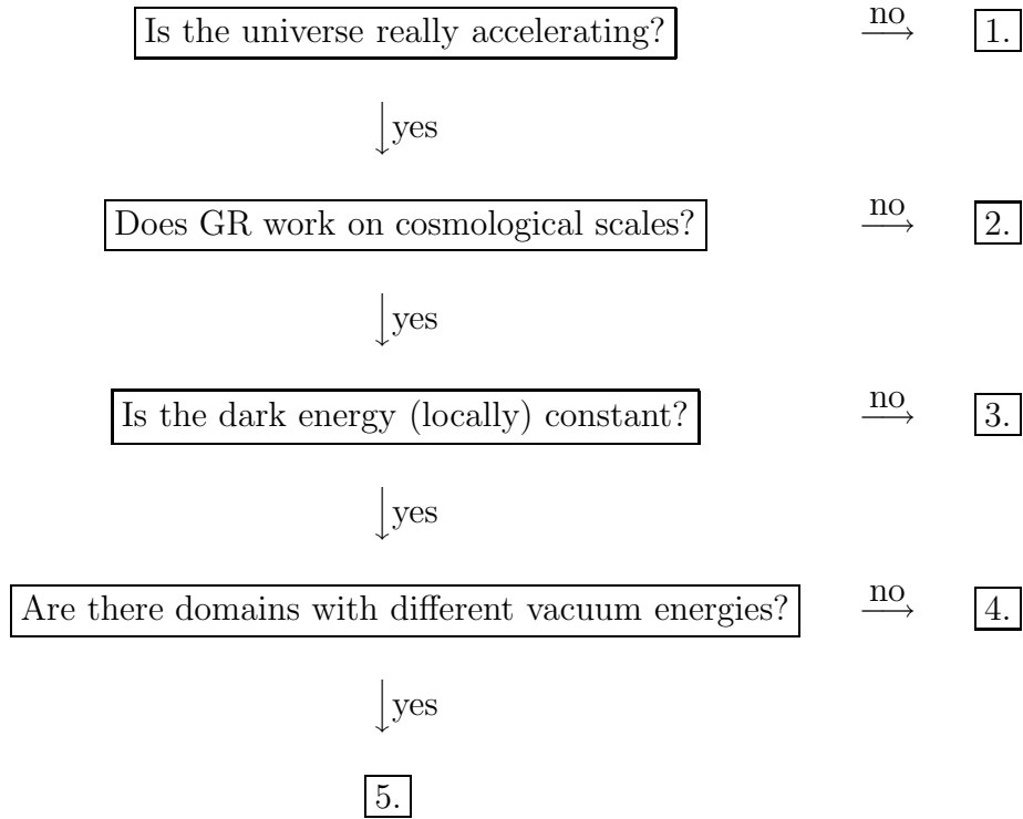
Figure 2: A flowchart classifying reasons why the universe might be accelerating. The possibilities include: 1. Misinterpretation of the data; 2. Breakdown of general relativity; 3. Dynamical dark energy; 4. Unique vacuum energy; 5. Environmental selection.
