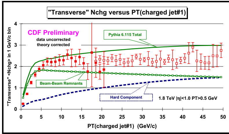
Figure 9: Data on the average number of charged particles ( p_T > 0.5 GeV/c, |\eta| < 1 ) in the “transverse” region defined in FIG. 3 as a function of the transverse momentum of the leading charged jet compared with the QCD Monte-Carlo predictions of PYTHIA 6.115 (default parameters and p_T(\text{hard}) > 3 GeV/c). The predictions of PYTHIA are divided into two categories: charged particles that arise from the break-up of the beam and target ( beam-beam remnants ), and charged particles that result from the outgoing jets plus initial and final-state radiation ( hard scattering component ). For PYTHIA the “beam-beam remnants” include contributions from multiple parton scattering. The theory curves are corrected for the track finding efficiency and have an error ( statistical plus systematic ) of around 5%.
