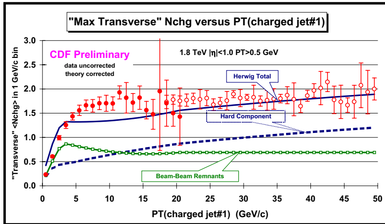
Figure 14: Data on the average number of “transMAX” charged particles ( p_T > 0.5 GeV/c, |\eta| < 1 ) as a function of the transverse momentum of the leading charged jet compared with the QCD Monte-Carlo predictions of HERWIG 5.9 (default parameters and p_T(\text{hard}) > 3 GeV/c). The predictions of HERWIG are divided into two categories: charged particles that arise from the break-up of the beam and target ( beam-beam remnants ), and charged particles that result from the outgoing jets plus initial and final-state radiation ( hard scattering component ). The theory curves are corrected for the track finding efficiency and have an error ( statistical plus systematic ) of around 5%.
