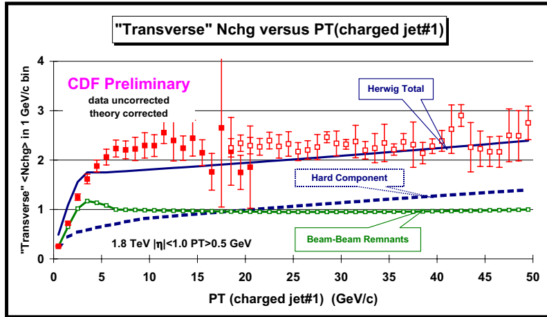
Figure 8: Data on the average number of charged particles ( p_T > 0.5 GeV/c, |\eta| < 1 ) in the “transverse” region defined in FIG. 3 as a function of the transverse momentum of the leading charged jet compared with the QCD Monte-Carlo predictions of HERWIG 5.9 (default parameters and p_T(\text{hard}) > 3 GeV/c). The predictions of HERWIG are divided into two categories: charged particles that arise from the break-up of the beam and target ( beam-beam remnants ), and charged particles that result from the outgoing jets plus initial and final-state radiation ( hard scattering component ). The theory curves are corrected for the track finding efficiency and have an error ( statistical plus systematic ) of around 5%.
