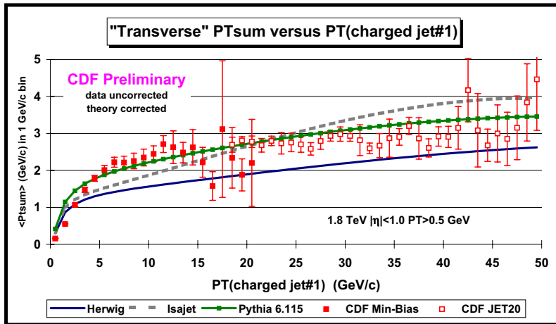
Figure 6: Data on the average scalar p_T sum of charged particles ( p_T > 0.5 GeV/c, |\eta| < 1 ) in the “transverse” region defined in FIG. 3 as a function of the transverse momentum of the leading charged jet compared with the QCD Monte-Carlo predictions of HERWIG 5.9, ISAJET 7.32, and PYTHIA 6.115 with their default parameters and with p_T(\text{hard}) > 3 GeV/c. Each point corresponds to the \langle P_{T\text{sum}} \rangle in a 1 GeV/c bin. The solid (open) points are the Min-Bias (JET20) data. The theory curves are corrected for the track finding efficiency and have an error ( statistical plus systematic ) of around 5%.
