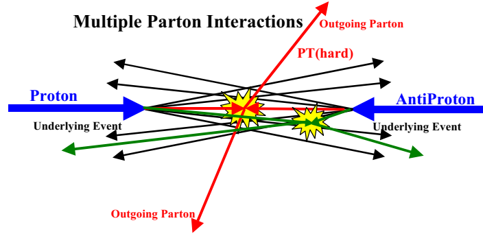
Figure 2: Illustration of the way PYTHIA models the “underlying event” in proton-antiproton collision by including multiple parton interactions. In addition to the hard 2-to-2 parton-parton scattering with transverse momentum, p_T(\text{hard}) , there is a second “semi-hard” 2-to-2 parton-parton scattering that contributes particles to the “underlying event”.
