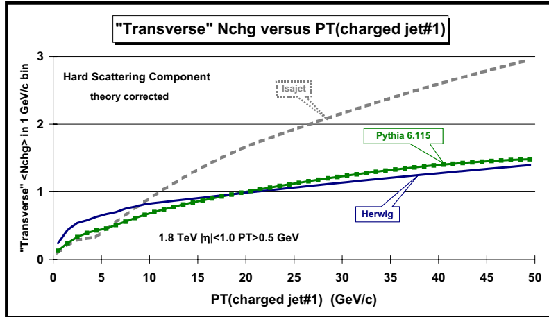
Figure 10: The “hard scattering” component ( outgoing jets plus initial and final-state radiation ) of the number of charged particles ( p_T > 0.5 GeV/c, |\eta| < 1 ) in the “transverse” region defined in FIG. 3 as a function of the transverse momentum of the leading charged jet from the QCD Monte-Carlo predictions of HERWIG 5.9, ISAJET 7.32, and PYTHIA 6.115 with their default parameters and with p_T(\text{hard}) > 3 GeV/c. The curves are corrected for the track finding efficiency and have an error ( statistical plus systematic ) of around 5%.
