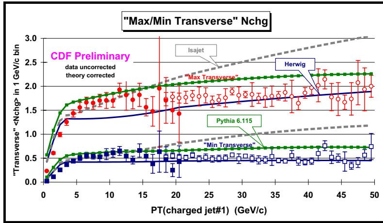
Figure 12: Data on the average number of “transMAX” and “transMIN” charged particles ( p_T > 0.5 GeV/c, |\eta| < 1 ) as a function of the transverse momentum of the leading charged jet compared with the QCD Monte-Carlo predictions of HERWIG 5.9, ISAJET 7.32, and PYTHIA 6.115 with their default parameters and with p_T(\text{hard}) > 3 GeV/c. The solid (open) points are the Min-Bias (JET20) data. The theory curves are corrected for the track finding efficiency and have an error (statistical plus systematic) of around 5%.
