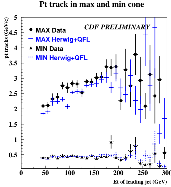
Figure 21: Data on the average scalar p_T sum of charged particles ( p_T > 0.4 \text{ GeV/c} , |\eta| < 1 ) within the maximum (MAX) and minimum (MIN) “transverse cones” defined in FIG. 20 versus the transverse energy of the leading ( highest E_T ) “calorimeter jet” compared with the QCD Monte-Carlo model predictions HERWIG 5.9 ( default parameters ).
