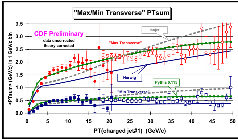
Figure 13: Data on the average scalar p_T sum of the “transMAX” and “transMIN” charged particles ( p_T > 0.5 GeV/c, |\eta| < 1 ) as a function of the transverse momentum of the leading charged jet compared with the QCD Monte-Carlo predictions HERWIG 5.9, ISAJET 7.32, and PYTHIA 6.115 with their default parameters and with p_T(\text{hard}) > 3 GeV/c. The solid (open) points are the Min-Bias (JET20) data. The theory curves are corrected for the track finding efficiency and have an error ( statistical plus systematic ) of around 5%.
