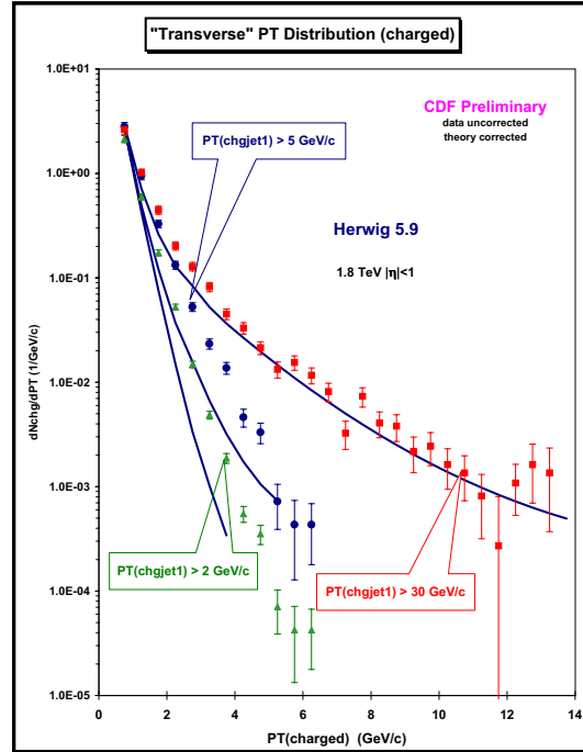
Figure 17: Data on the transverse momentum distribution of charged particles ( p_T > 0.5 \text{ GeV}/c , |\eta| < 1 ) in the “transverse” region for P_T(\text{chgjet}\#1) > 2 \text{ GeV}/c , 5 \text{ GeV}/c , and 30 \text{ GeV}/c , where \text{chgjet}\#1 is the leading charged particle jet. Each point corresponds to dN_{\text{chg}}/dp_T and the integral of the distribution gives the average number of charged particles in the transverse region, \langle N_{\text{chg}}(\text{transverse}) \rangle . The data are compared with the QCD Monte-Carlo model predictions of HERWIG 5.9 (default parameters and p_T(\text{hard}) > 3 \text{ GeV}/c ). The theory curves are corrected for the track finding efficiency and have an error ( statistical plus systematic ) of around 5%.
