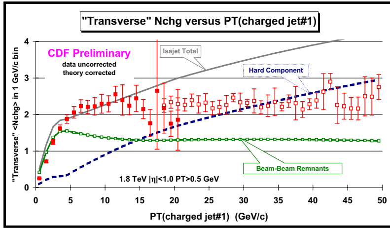
Figure 7: Data on the average number of charged particles ( p_T > 0.5 GeV/c, |\eta| < 1 ) in the “transverse” region defined in FIG. 3 as a function of the transverse momentum of the leading charged jet compared with the QCD Monte-Carlo predictions of ISAJET 7.32 (default parameters and p_T(\text{hard}) > 3 GeV/c). The predictions of ISAJET are divided into two categories: charged particles that arise from the break-up of the beam and target ( beam-beam remnants ), and charged particles that result from the outgoing jets plus initial and final-state radiation ( hard scattering component ). The theory curves are corrected for the track finding efficiency and have an error ( statistical plus systematic ) of around 5%.
