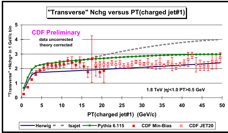
Figure 5: Data on the average number of charged particles ( p_T > 0.5 GeV/c, |\eta| < 1 ) in the “transverse” region defined in FIG. 3 as a function of transverse momentum of the leading charged jet compared with the QCD Monte-Carlo predictions of HERWIG 5.9, ISAJET 7.32, and PYTHIA 6.115 with their default parameters and with p_T(\text{hard}) > 3 GeV/c. Each point corresponds to the \langle N_{\text{chg}} \rangle in a 1 GeV/c bin. The solid (open) points are the Min-Bias (JET20) data. The theory curves are corrected for the track finding efficiency and have an error ( statistical plus systematic ) of around 5%.
