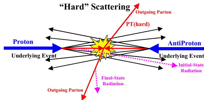
Figure 1: Illustration of the way QCD Monte-Carlo models simulate a proton-antiproton collision in which a “hard” 2-to-2 parton scattering with transverse momentum, p_T(\text{hard}) , has occurred. The resulting event contains particles that originate from the two outgoing partons ( plus initial and final-state radiation ) and particles that come from the breakup of the proton and antiproton (“beam-beam remnants”). The “underlying event” is everything except the two outgoing hard scattered “jets” and consists of the “beam-beam remnants” plus initial and final-state radiation. The “hard scattering” component consists of the outgoing two “jets” plus initial and final-state radiation.
