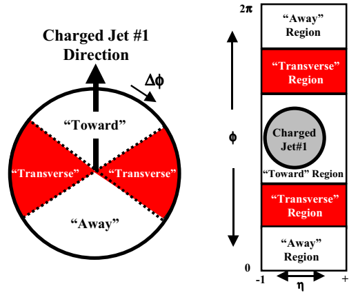
Figure 3: Illustration of correlations in azimuthal angle \Delta\phi relative to the direction of the leading charged jet in the event, \text{chgjet}\#1 . The angle \Delta\phi = \phi - \phi_{\text{chgjet}\#1} is the relative azimuthal angle between charged particles and the direction of \text{chgjet}\#1 . The “toward” region is defined by |\Delta\phi| < 60^\circ and |\eta| < 1 , while the “away” region is |\Delta\phi| > 120^\circ and |\eta| < 1 . The “transverse” region is defined by 60^\circ < |\Delta\phi| < 120^\circ and |\eta| < 1 . Each region has an area in \eta - \phi space of 4\pi/3 .
