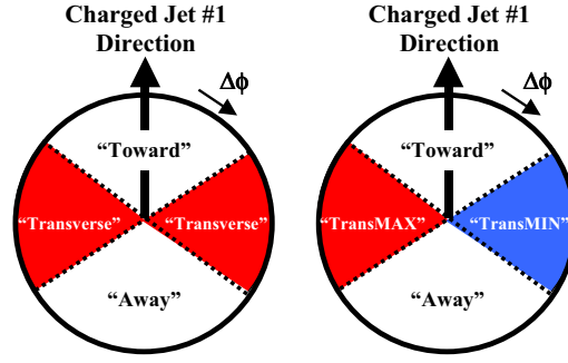
Figure 11: Illustration of correlations in azimuthal angle \Delta\phi relative to the direction of the leading charged jet in the event, \text{chgjet}\#1 . The angle \Delta\phi = \phi - \phi_{\text{chgjet}\#1} is the relative azimuthal angle between charged particles and the direction of \text{chgjet}\#1 . On an event by event basis, we define “transMAX” (“transMIN”) to be the maximum (minimum) of the two “transverse” pieces, 60^\circ < \Delta\phi < 120^\circ and |\eta| < 1 , and 60^\circ < -\Delta\phi < 120^\circ and |\eta| < 1 . “TransMAX” and “transMIN” each have an area in \eta - \phi space of 2\pi/3 . The sum of “TransMAX” and “transMIN” is the total “transverse” region with area 4\pi/3 .
