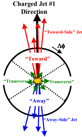
Figure 4: Illustration of the topology of an average proton-antiproton collision in which a “hard” 2-to-2 parton scattering has occurred. The “toward” region as defined in FIG. 3 contains the leading charged particle “jet”, while the “away” region, on the average, contains the “away-side” jet. The “transverse” region is perpendicular to the plane of the hard 2-to-2 scattering and is very sensitive to the “underlying event”.
