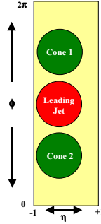
Figure 20: Illustration of “transverse cones” with radius in \eta - \phi space of R = 0.7 which are located at the same pseudorapidity as the leading jet but with azimuthal angle \Delta\phi = +90^\circ and \Delta\phi = -90^\circ relative to the leading jet. Each “transverse cone” has an area in \eta - \phi space of \pi R^2 = 0.49\pi .
