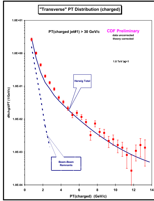
Figure 19: Data on the transverse momentum distribution of charged particles ( p_T > 0.5 GeV/c, |\eta| < 1 ) in the “transverse” region for P_T(\text{chgjet}\#1) > 30 GeV/c compared with the QCD Monte-Carlo model predictions of HERWIG 5.9 (default parameters and p_T(\text{hard}) > 3 GeV/c). The theory curves are corrected for the track finding efficiency and have an error ( statistical plus systematic ) of around 5%. The solid curve is the total (“hard scattering” plus “beam-beam remnants”) and the dashed curve shows the contribution arising from the break-up of the beam particles (“beam-beam remnants”).
