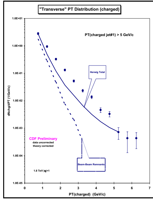
Figure 18: Data on the transverse momentum distribution of charged particles ( p_T > 0.5 GeV/c, |\eta| < 1 ) in the “transverse” region for P_T(\text{chgjet}\#1) > 5 GeV/c compared with the QCD Monte-Carlo model predictions of HERWIG 5.9 (default parameters and p_T(\text{hard}) > 3 GeV/c). The theory curves are corrected for the track finding efficiency and have an error ( statistical plus systematic ) of around 5%. The solid curve is the total (“hard scattering” plus “beam-beam remnants”) and the dashed curve shows the contribution arising from the break-up of the beam particles (“beam-beam remnants”).
