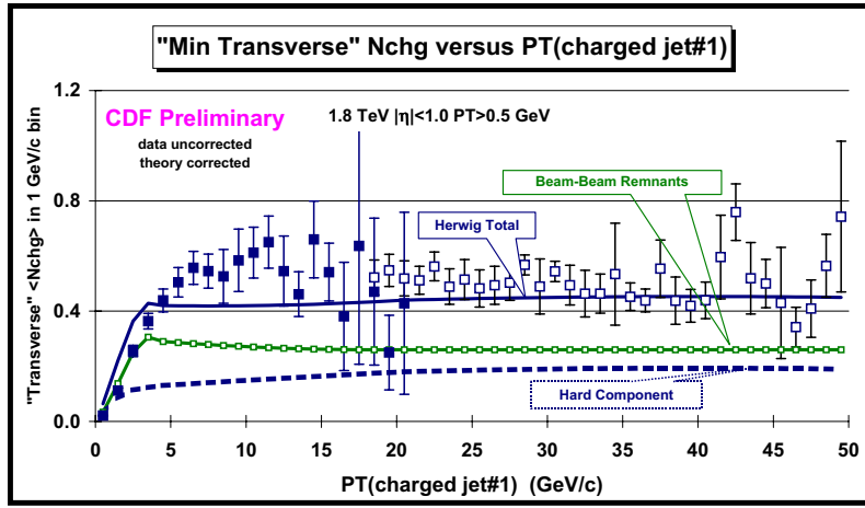
Figure 15: Data on the average number of “transMIN” charged particles ( p_T > 0.5 GeV/c, |\eta| < 1 ) as a function of the transverse momentum of the leading charged jet compared with the QCD Monte-Carlo predictions of HERWIG 5.9 (default parameters and p_T(\text{hard}) > 3 GeV/c). The predictions of HERWIG are divided into two categories: charged particles that arise from the break-up of the beam and target ( beam-beam remnants ), and charged particles that result from the outgoing jets plus initial and final-state radiation ( hard scattering component ). The theory curves are corrected for the track finding efficiency and have an error ( statistical plus systematic ) of around 5%.
