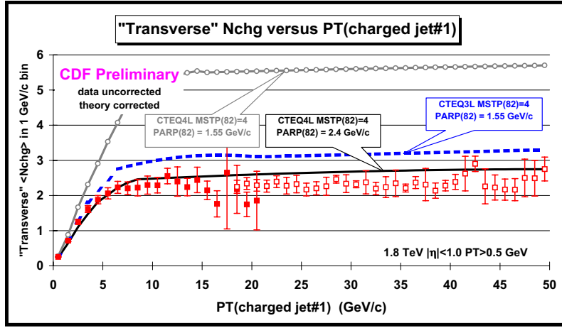
Figure 23: Data on the average number of charged particles ( p_T > 0.5 GeV/c, |\eta| < 1 ) in the “transverse” region as a function of the transverse momentum of the leading charged jet compared with the QCD Monte-Carlo predictions of PYTHIA 6.115 with different structure functions and different multiple parton interaction parameters and with p_T(\text{hard}) > 0 GeV/c. The theory curves are corrected for the track finding efficiency and have an error ( statistical plus systematic ) of around 5%.
