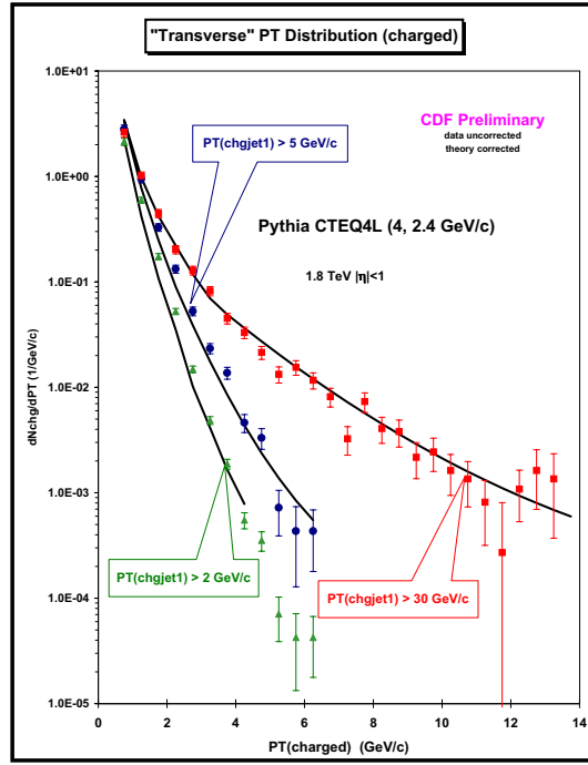
Figure 28: Data on the transverse momentum distribution of charged particles ( p_T > 0.5 GeV/c, |\eta| < 1 ) in the “transverse” region for P_T(\text{chgjet}\#1) > 2 GeV/c, 5 GeV/c, and 30 GeV/c, where chgjet#1 is the leading charged particle jet. Each point corresponds to dN_{\text{chg}}/dp_T and the integral of the distribution gives the average number of charged particles in the transverse region, \langle N_{\text{chg}}(\text{transverse}) \rangle . The data are compared with the QCD Monte-Carlo model predictions of PYTHIA 6.115 ( tuned version , CTEQ4L, MSTP(82) = 4, PARP(82) = 1.4 GeV/c, p_T(\text{hard}) > 0 GeV/c). The theory curves are corrected for the track finding efficiency and have an error ( statistical plus systematic ) of around 5%.
