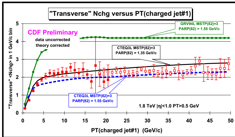
Figure 22: Data on the average number of charged particles ( p_T > 0.5 \text{ GeV}/c , |\eta| < 1 ) in the “transverse” region as a function of the transverse momentum of the leading charged jet compared with the QCD Monte-Carlo predictions of PYTHIA 6.115 with different structure functions and different multiple parton interaction parameters and with p_T(\text{hard}) > 0 \text{ GeV}/c . The theory curves are corrected for the track finding efficiency and have an error ( statistical plus systematic ) of around 5%.
