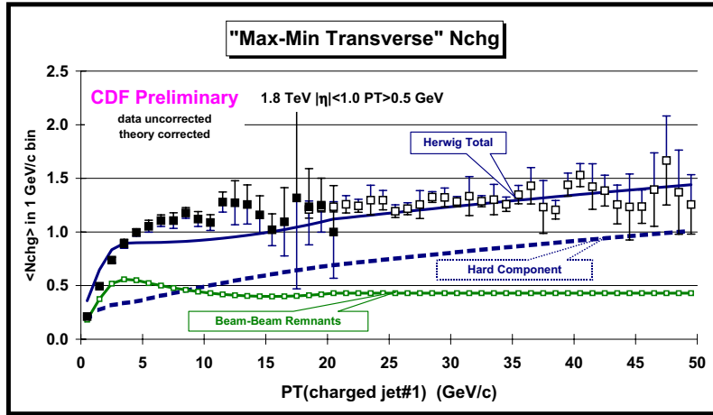
Figure 16: Data on the average difference, “transMAX” minus “transMIN”, for the number of charged particles ( p_T > 0.5 GeV/c, |\eta| < 1 ) as a function of the transverse momentum of the leading charged jet compared with the QCD Monte-Carlo predictions of HERWIG 5.9 (default parameters and p_T(\text{hard}) > 3 GeV/c). The predictions of HERWIG are divided into two categories: charged particles that arise from the break-up of the beam and target ( beam-beam remnants ), and charged particles that result from the outgoing jets plus initial and final-state radiation ( hard scattering component ). The theory curves are corrected for the track finding efficiency and have an error ( statistical plus systematic ) of around 5%.
