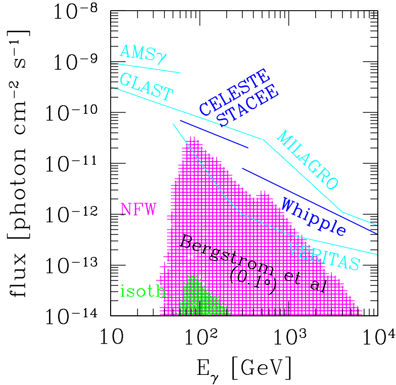
Figure 3: Gamma-ray line flux expected from neutralino annihilations in the galactic halo from the direction of the galactic center compared with experimental sensitivities. The region marked “NFW” is for a cuspy halo, and the region marked “isoth.” is for a standard halo. Theoretical models from Bergström et al. [1998] . Figure from Gondolo [2000a] .
