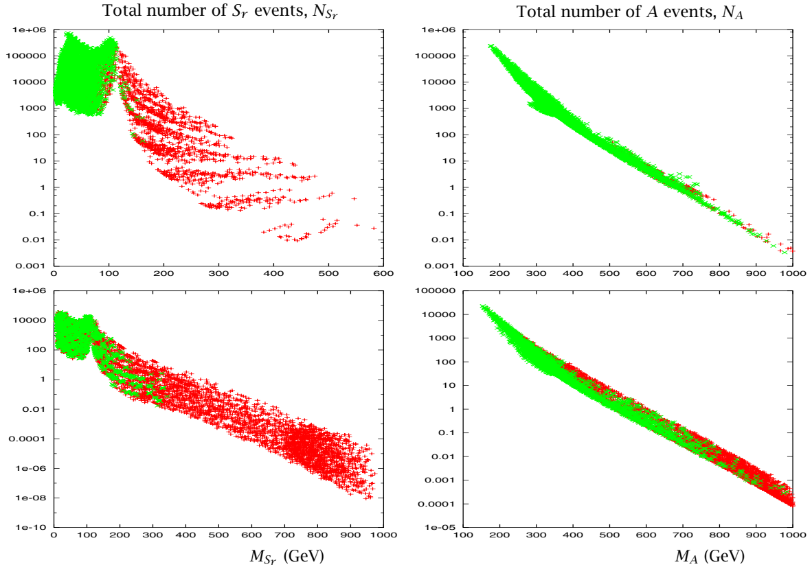
Figure 1: Total number of events produced through processes (2) at the Tevatron (Run II) after 15 \text{ fb}^{-1} in the NMSSM (upper plots) and nMSSM (lower plots) for the CP-even singlet S_r (left plots) and the CP-odd non-singlet A (right plots) as a function of the produced Higgs mass. (For an explanation of the colour coding, see the text).
