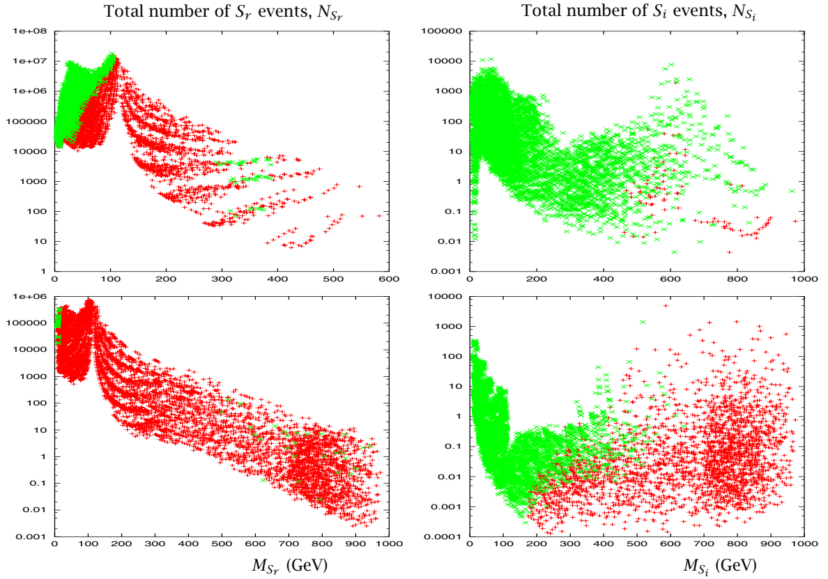
Figure 2: As Fig. 1 for the CP-even singlet S_r (left plots) and the CP-odd singlet S_i (right plots), at LHC after 300 fb -1 .
