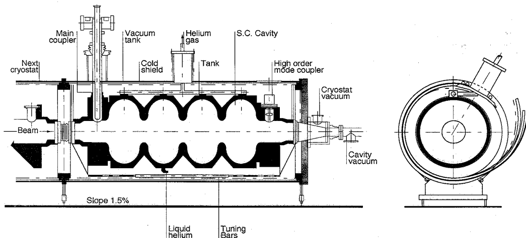
FIG. 1: Superconducting cavity in module.
