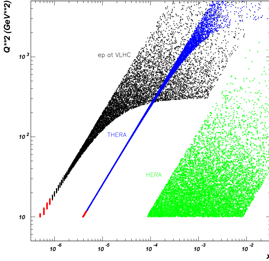
FIG. 1: Kinematics at HERA, THERA, and epVLHC, indicating where saturation is expected to occur.
