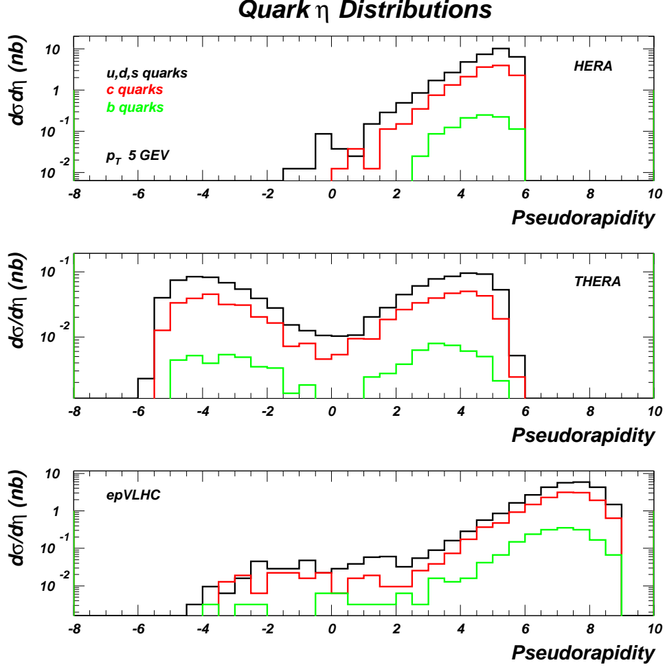
FIG. 3: \eta distributions of quarks at HERA, THERA, and epVLHC.
