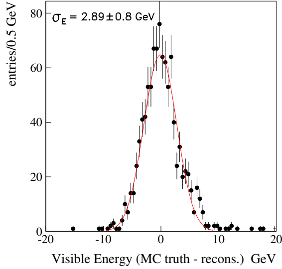
Figure 3: The visible mass resolution for q\bar{q} Z decays at rest.
