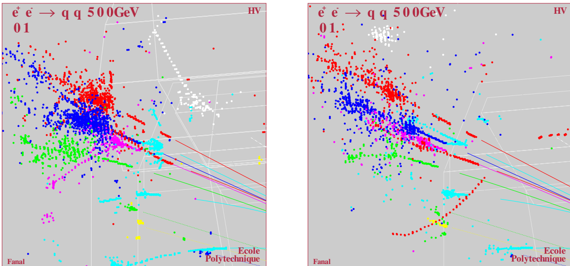
Figure 2: The same di-jet for a digital-steel (left) or for a digital-tungsten (right) HCAL
