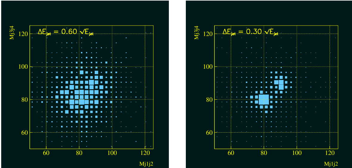
Figure 1: Impact of the jet energy resolution on the WW/ZZ separation, when \alpha (see text) goes from 0.6 (left) to 0.3 (right).
