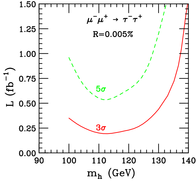
Figure 9: Integrated luminosity (in \text{fb}^{-1} ) needed for observing the two-body decay channels \tau \rightarrow \rho\nu_\tau and \tau \rightarrow \pi\nu_\tau at 3\sigma (solid) and 5\sigma (dashed) significance. Beam energy resolution R = 0.005\% and a 25% polarization are assumed.
