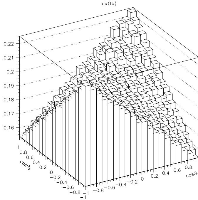
Figure 7: Double differential distribution for \mu^-\mu^+ \rightarrow h \rightarrow \tau^-\tau^+ \rightarrow \rho^-\nu_\tau\rho^+\bar{\nu}_\tau . \sqrt{s} = m_h = 120 GeV is assumed. Initial \mu^\mp beam polarizations are taken to be P_- = P_+ = 0.25 . The Higgs production cross section is convoluted with Gaussian energy distribution for a resolution R = 0.05\% .
