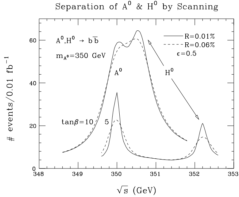
Figure 11: Separation of A and H signals for \tan \beta = 5 and 10 . From Ref. [10].
