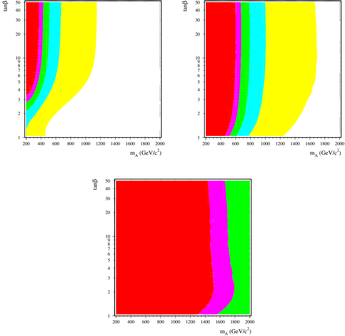
Figure 4: The m_{A^0} - \tan \beta discrimination from the measurements at (a) LHC(300 fb ^{-1} )+LC(500 fb ^{-1} ), (b) 0.2 fb ^{-1} at a muon collider, and (c) 10 fb ^{-1} at a muon collider. The exclusion regions (starting from the left) are > 5\sigma , 4 - 5\sigma , 3 - 4\sigma , 2 - 3\sigma , and 1 - 2\sigma . From Ref. [13].
