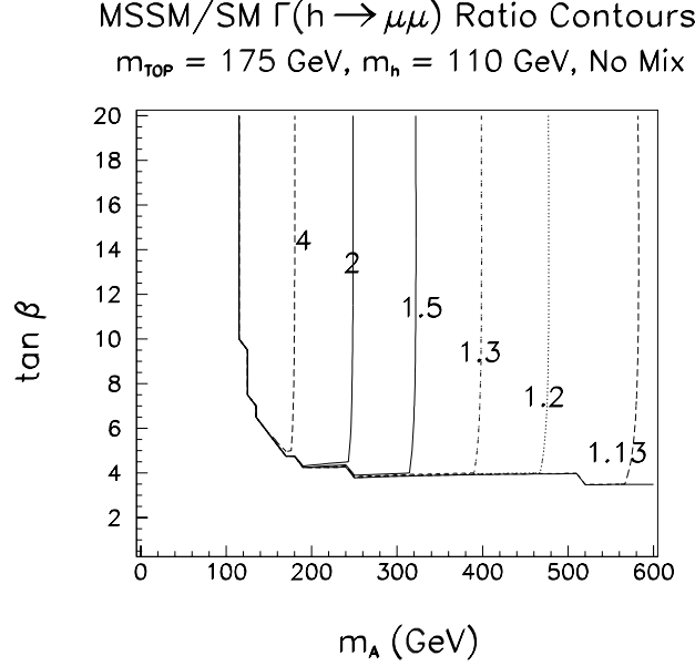
Figure 6: Contours in (m_{A^0}, \tan \beta) parameter space for \Gamma(h^0 \rightarrow \mu^+ \mu^-)/\Gamma(h_{SM} \rightarrow \mu^+ \mu^-) . We have assumed a no-mixing SUSY scenario and employed m_{h^0} = m_{h_{SM}} = 110 \text{ GeV} . For maximal mixing, there is little change in the contours — only the size of the allowed range is altered. From [21].
