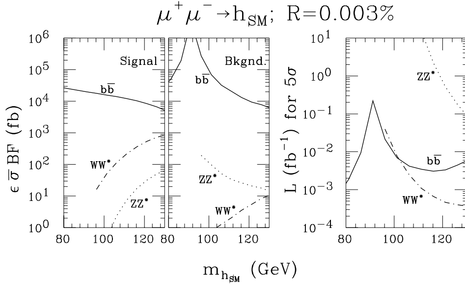
Figure 3: The SM Higgs cross sections and backgrounds in b\bar{b} , WW^* and ZZ^* . Also shown is the luminosity needed for a 5 standard deviation detection in b\bar{b} . From Ref. [10].
