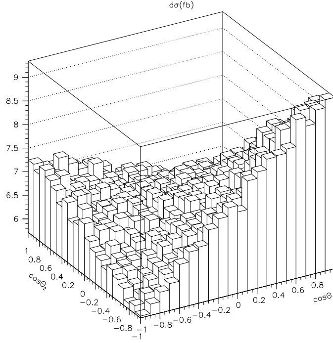
Figure 8: Double differential distribution for \mu^-\mu^+ \rightarrow \gamma^*/Z^* \rightarrow \tau^-\tau^+ \rightarrow \rho^-\nu_\tau\rho^+\bar{\nu}_\tau . \sqrt{s} = 120 GeV is assumed. Initial \mu^\pm beam polarizations are taken to be P_- = P_+ = 0.25 . The SM production cross section is convoluted with Gaussian energy distribution for a resolution R = 0.05\% .
