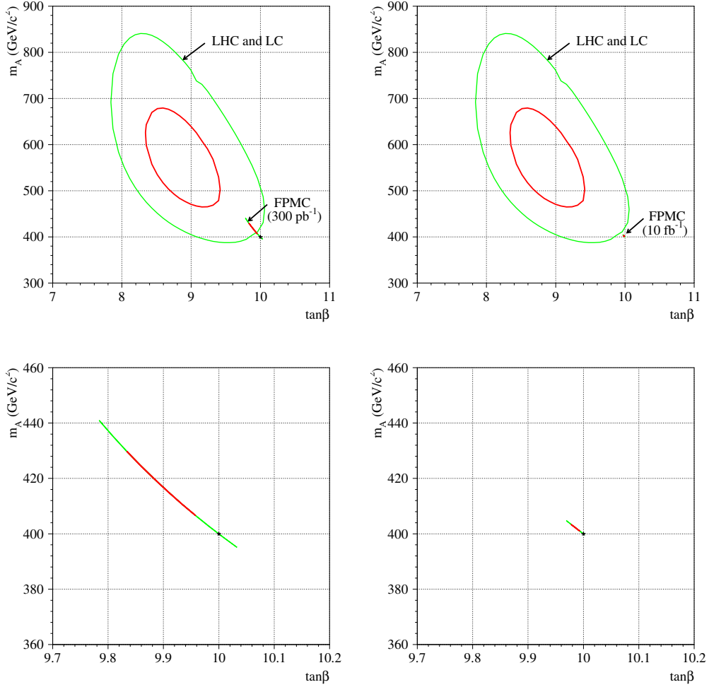
Figure 5: The implications of the h^0 scan for the MSSM [m_{A^0}, \tan\beta] parameter space, assuming all other SUSY parameters are known. In the lower figures, we illustrate the results that would emerge were there no systematic theoretical uncertainties in the m_{h^0} computation in terms of input SUSY parameters. The experimental error of m_{h^0} at a muon collider would not significantly broaden this line. The LH (RH) lower figure shows the extent to which the location along this line would be fixed by L = 0.1 \text{ fb}^{-1} ( L = 10 \text{ fb}^{-1} ) muon collider measurements of N(\mu^+\mu^- \rightarrow h \rightarrow b\bar{b}) and \Gamma_h^{\text{tot}} , with the former being the dominant ingredient given its much smaller error. In the upper two figures, the restrictions (1 and 2 \sigma ellipses) that would emerge from LHC+LC measurements (including the measurement of m_{h^0} with accuracy of order \pm 30 \text{ MeV} ) are shown. (Note the much more coarse scale of the upper figures.) These figures are from Ref. [13]. Unfortunately, the systematic error ( \gtrsim \pm 100 \text{ MeV} , at best) expected for the m_{h^0} computation in terms of the input SUSY parameters will cause the potential muon collider lines of the lower figures to turn into ellipses similar in size to the LHC+LC ellipses and will increase the size of the LHC+LC ellipses significantly.
