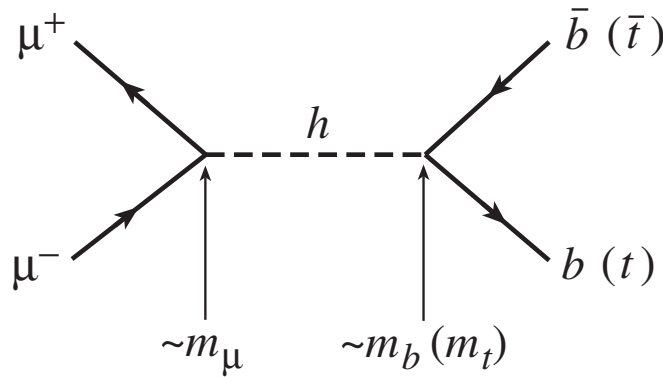
Figure 1: Feynman diagram for s -channel production of a Higgs boson.
