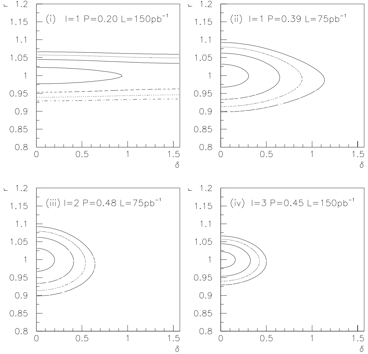
Figure 12: Contours at \Delta\chi^2 = 1, 4, 6.635, 9 for the \hat{a} and \hat{b} measurement for a SM Higgs ( \hat{a} = 1, \hat{b} = 0 ) with m_{h_{SM}} = 110 GeV for the four luminosity/bunch-merging options outlined in the text. Here, \delta = \tan^{-1} \frac{\hat{b}}{\hat{a}} and r = \sqrt{\hat{a}^2 + \hat{b}^2} . For small \delta , \frac{\hat{b}}{\hat{a}} \sim \delta .
