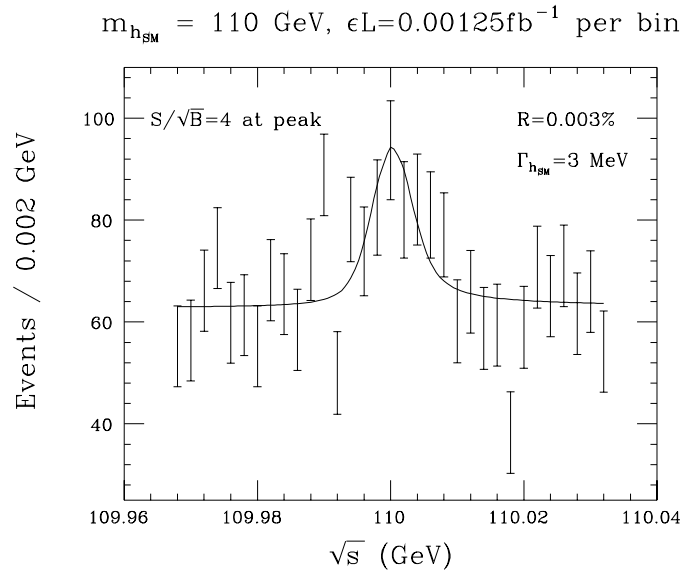
Figure 2: Number of events and statistical errors in the b\bar{b} final state as a function of \sqrt{s} in the vicinity of m_{h_{SM}} = 110 GeV, assuming R = 0.003\% , and \epsilon L = 0.00125 \text{ fb}^{-1} at each data point.
