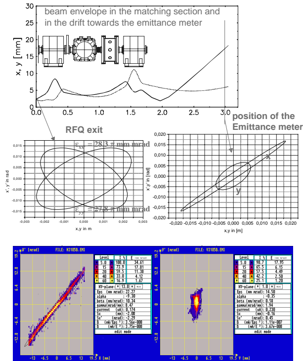
Figure 6: Calculated beam envelope in the matching section and towards the emittance meter and resulting emittances in comparison with measurements.
