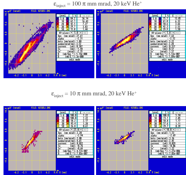
Figure 4: Measured beam emittances from the RFQ for different injection emittances.
