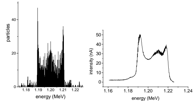
Figure 5: Measured energy spectrum (right) in comparison with PARMTEQ calculations for the design rod voltage.
