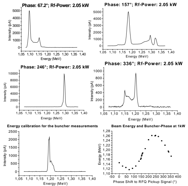
Figure 7: Energy spectra of the re-buncher at different phases relative to the RFQ pick up signal. The figures at the bottom show the energy peak out of the RFQ and the energy gain of the beam in dependence on the buncher phase.
