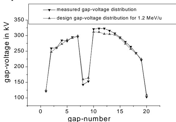
Figure 8: Perturbation measurement of the gap voltage distribution for the 1.2 MeV/u mode
