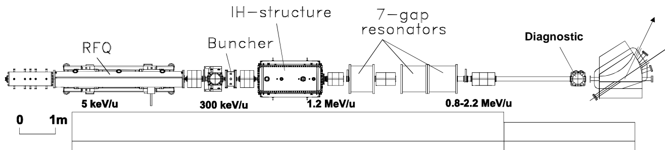
Figure 1: Lay-out of the REX-ISOLDE linear accelerator
