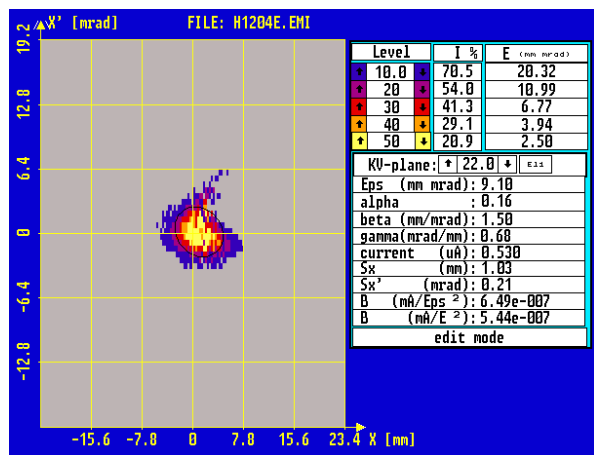
Figure 2: Measured beam emittance from the REXEBIS with 1ms confinement time and 20 kV platform potential.
