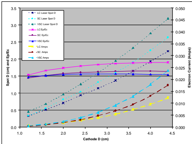
Figure 3: Spot D, electron current, and Epeak/Ecathode plotted as a function of cathode diameter for three cathode lengths
