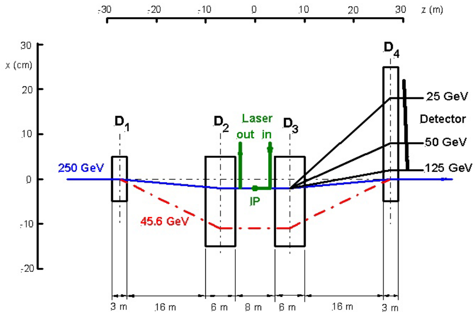
Upstream Polarimeter Chicane
