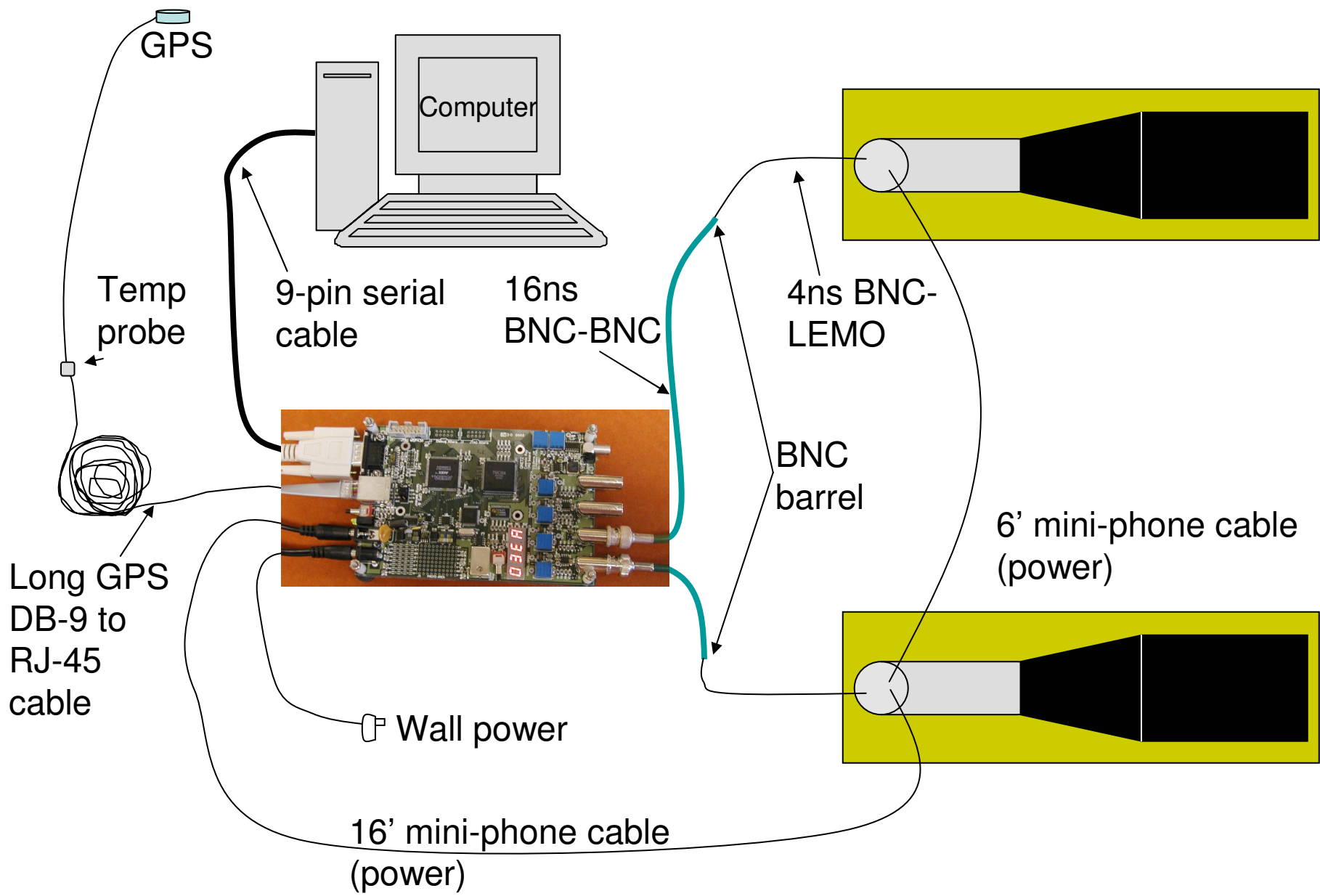
Cosmic Ray Telescope Layout
