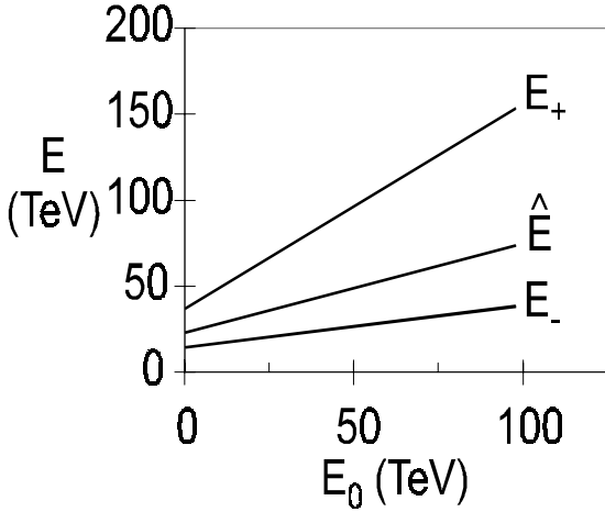
FIG. 2: Optimal RLHC energy \hat{E} given by the peak position of the curves in Fig. 1. Also shown are the energies at which the "physics per buck" has fallen to 90% of its optimum value.
