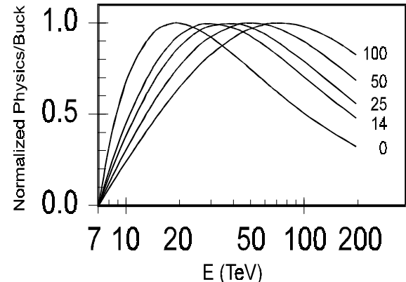
FIG. 1: Normalized "physics per buck" for the RLHC as a function of its energy, as given by Eq. 3 for the values of E_0 indicated (in TeV), using the LHC energy of E_1 = 7 \text{ TeV} .
