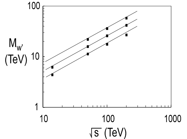
FIG. 3: The points show the mass reach as a function of proton-proton center-of-mass energy for luminosities of 10^{33} , 10^{34} and 10^{35} \text{ cm}^2 \text{ sec}^{-1} , under the assumptions described in the text. (The 14-TeV point for 10^{35} is unavailable.) The straight lines are given by Eq. 4 for these three luminosities.
