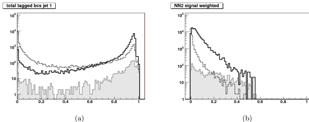
Figure 4.6: Neutrino channel: (a) Flavour tag 'c with b only background' for the first jet; (b) \text{NN}_{Higgs-signal} output. Solid curves are SM background, dashed curves are inclusive Higgs sample and filled histograms are the signal.
