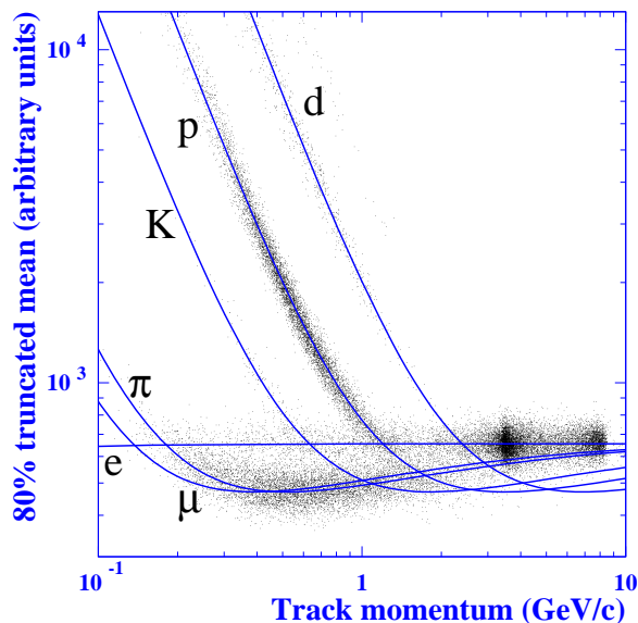
Figure 2.3: Drift Chamber dE/dx as a function of particle momentum. The scatter points are from beam scan data and the curves are appropriately parameterized Bethe-Bloch curves. The letters have their usual meanings, labelling the curves muon, electron, pion, kaon, proton and deuteron respectively.
