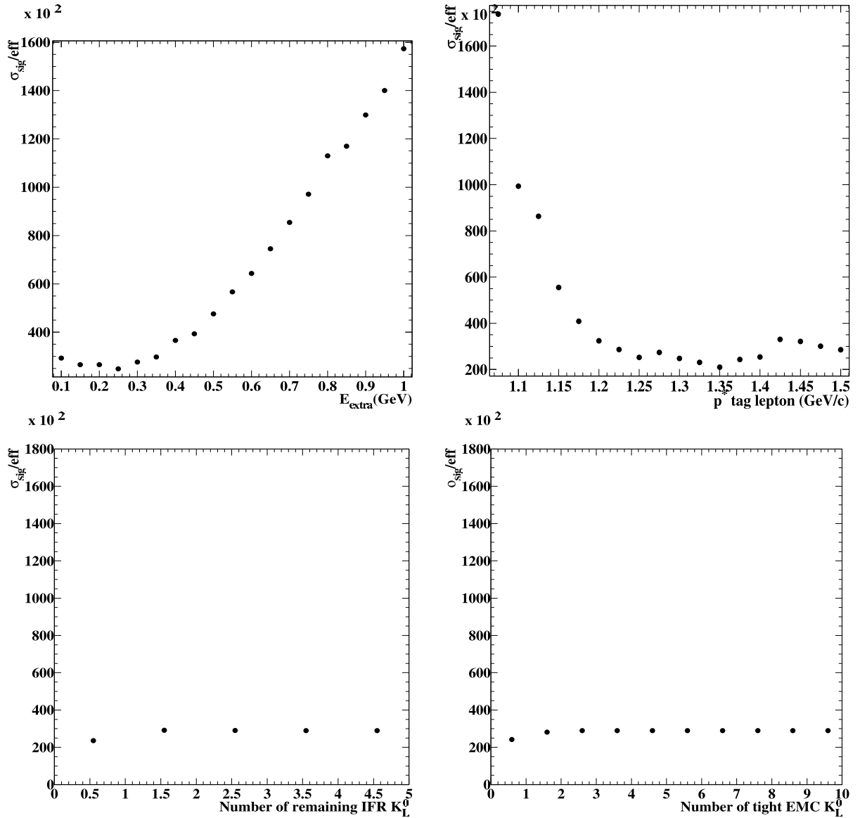
Figure 6.13: E_{\text{sig}}/\epsilon (as defined in the text) is plotted for E_{\text{extra}} , p^*_{\text{tag lepton}} and Number of tight K_L^0 candidates.
