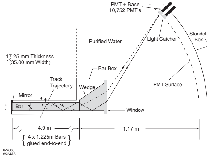
Figure 3.11: Schematic of the DIRC fused silica radiator bar and imaging region.
