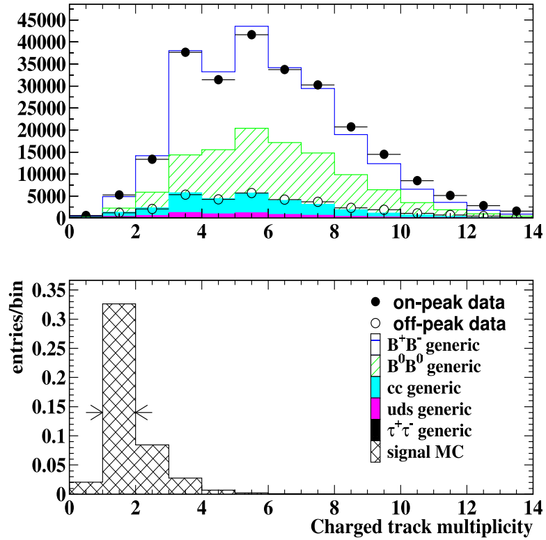
Figure 6.2: A plot of the number of remaining tracks after all the tag side particles have been removed from the event. All Monte Carlo ( B\bar{B} , q\bar{q} ( q = u, d, s or c ) and \tau^+ \tau^- ), onpeak and offpeak data are plotted. Distributions are scaled to the onpeak data luminosity. The B^+ \rightarrow K^+ \nu \bar{\nu} signal Monte Carlo is plotted for comparison. The arrow corresponds to the cut applied.
