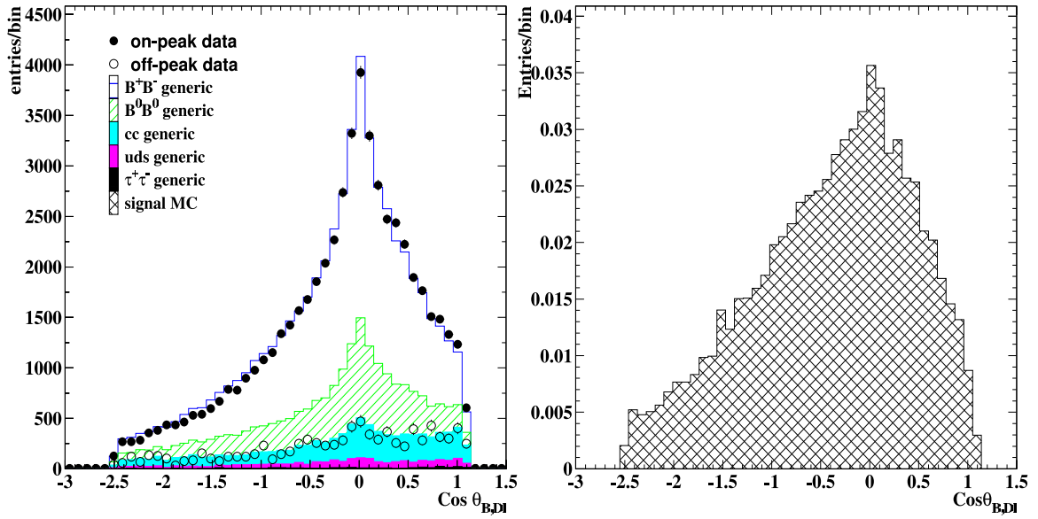
Figure 5.4: A plot of the \cos \theta_{B,D\ell} for all modes using all MC ( B\bar{B} , q\bar{q} ( q = u, d, s or c ) and \tau^+\tau^- ), onpeak and offpeak data. All distributions are scaled to the onpeak data luminosity. The B^+ \rightarrow K^+\nu\bar{\nu} signal MC is plotted on the right.
