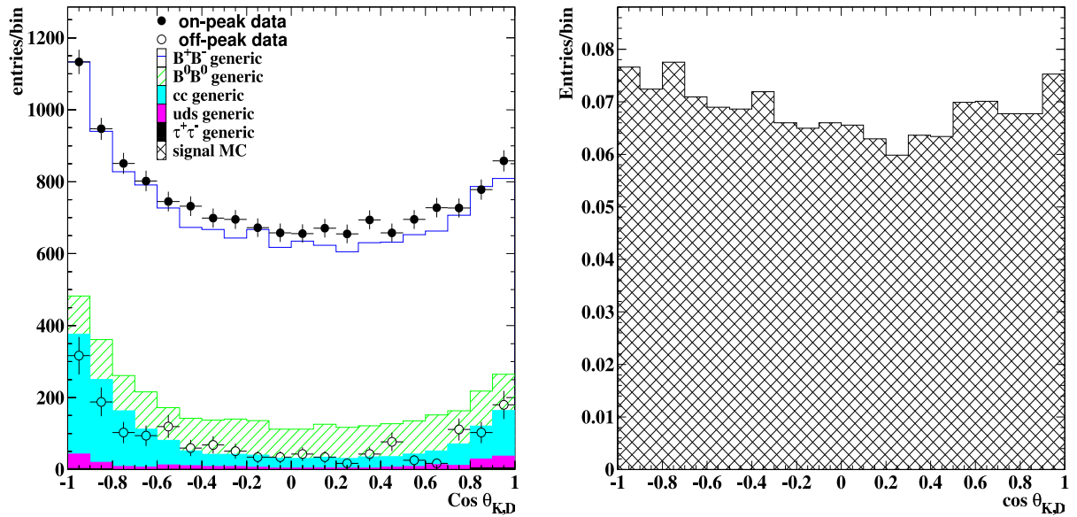
Figure 6.9: Cosine of the angle between the K and D meson used in the tag, \cos \theta_{K,D^0} . All Monte Carlo contributions and data are plotted (left) with the signal Monte Carlo plotted (right) for comparison.
