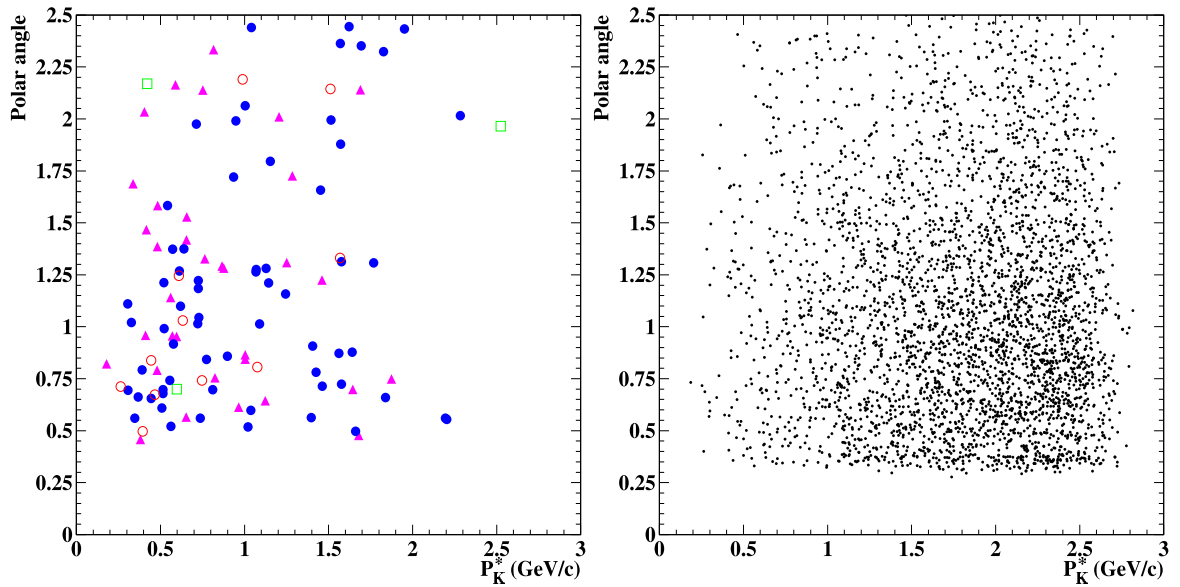
Figure 6.11: Scatter plots of the polar angle, \theta , versus momentum of the kaon candidate in the signal region. Generic B^+B^- are symbolised by solid (blue) circles, B^0\bar{B}^0 by the open (red) circles and c\bar{c} by the open (green) squares. On-peak data are plotted as solid (magenta) triangles. Signal Monte Carlo for B^+ \rightarrow K^+ \nu \bar{\nu} is plotted on the right.
