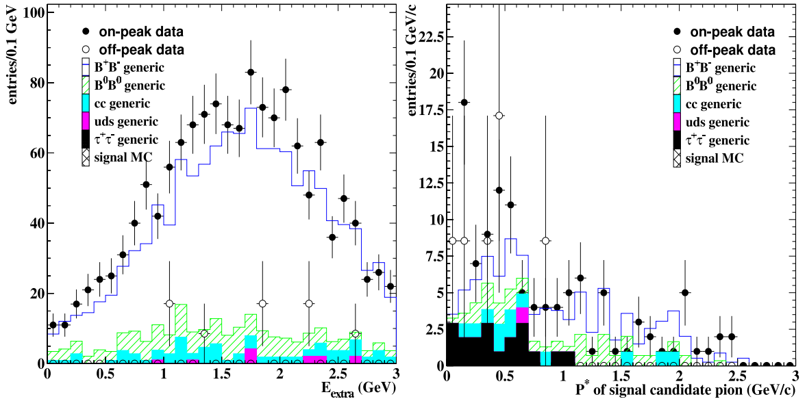
Figure 9.5: Unblinded distribution showing the E_{extra} and p_{\pi}^* for all Monte Carlo contributions with the data overlaid for the B^+ \rightarrow \pi^+ \nu \bar{\nu} channel. The p_{\pi}^* > 1.25 \text{ GeV}/c cut is applied to the E_{extra} plot and the E_{extra} < 0.25 \text{ GeV} is applied to the p_{\pi}^* distribution.
