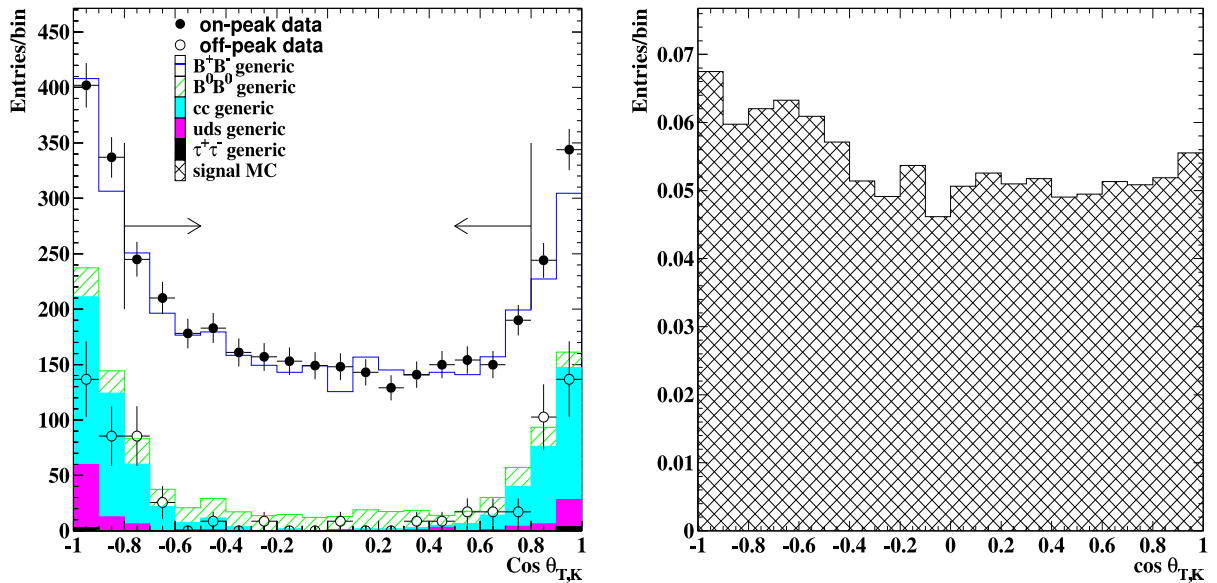
Figure 6.10: Cosine of the angle between the K and thrust axis of the rest of the event, \cos \theta_{\vec{T},K} . All Monte Carlo contributions and data are plotted (left) with the signal Monte Carlo plotted (right) for comparison.
