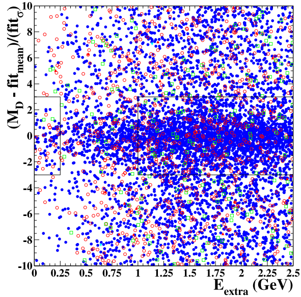
Figure 9.3: All background Monte Carlo distribution for B^+ \rightarrow \pi^+ \nu \bar{\nu} search showing number of sigma from the mean of the D^0 mass vs E_{extra} . The Monte Carlo is split up by type into B^+B^- (solid (blue) circles), B^0\bar{B}^0 (open (red) circles), c\bar{c} (open (green) squares) and uds (solid (red) triangles).
