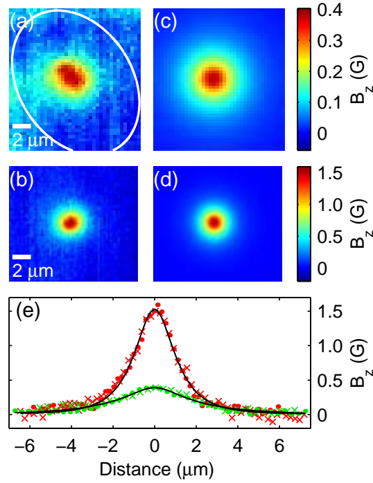
Figure 5.4: Scanning Hall probe vortex images and fits to a model described in the text (with z_0 = 0.8 \mu\text{m} ) in a \text{YBa}_2\text{Cu}_3\text{O}_{6.375} single crystal. (a) For T_c = 5.1 \text{ K} and T = 2.0 \text{ K} . The non-uniform shape was typical of vortices at this T_c . (b) For T_c = 14.7 \text{ K} and T = 4.0 \text{ K} . (c) 2D fit to image (a) within the white oval with best fit parameter s_{ab} = 1.86 \mu\text{m} . (d) 2D fit to image (b) with best fit parameter s_{ab} = 0.55 \mu\text{m} . Images and fits are displayed with a constant offset subtracted and color-scales corresponding to the bars at right. (e) Horizontal ( \times ) and vertical ( \bullet ) cross-sections through the vortex center in image (a) (green), image (b) (red), and corresponding fits (c) and (d) (black lines).
