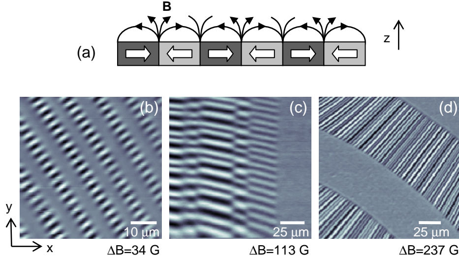
Figure 1.4: Images of magnetic bits taken with a 2\ \mu\text{m} Hall probe. (a) Schematic of bit magnetization and resulting field lines. (b) Image of bits spaced 1.69\ \mu\text{m} (sample courtesy of Shan Wang) at T = 4\ \text{K} . (c) Image of an old hard disk at room temperature. (d) Image of a floppy disk at room temperature. Hysteresis in the scanner at room temperature caused the tracks to appear curved. (For each image “ \Delta B ” gives the fullscale of the colormap.)
