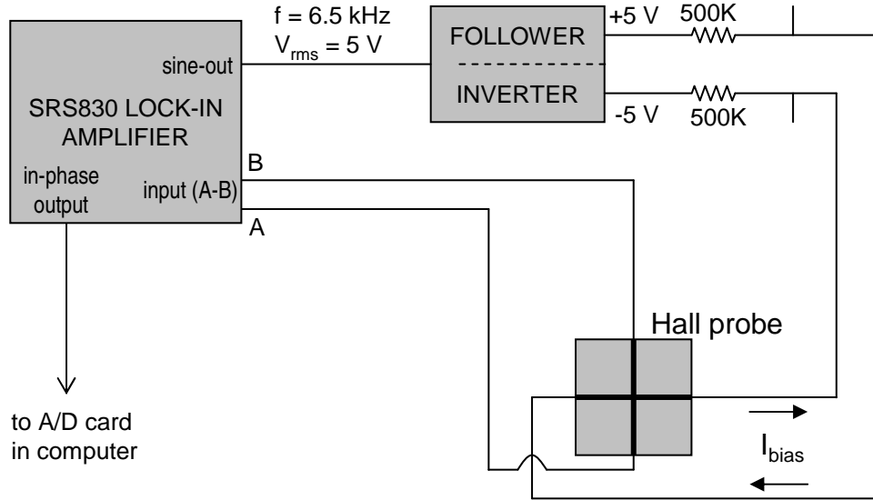
Figure 3.20: Diagram of the Hall probe electronics. The grounded gate of the Hall probe is not shown. The tees to the right of the 500K resistors allow the Hall probe to be grounded with BNC shorting caps.
