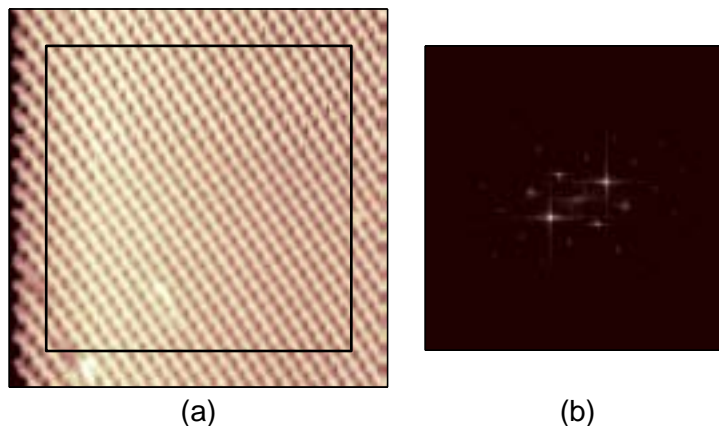
Figure 2.7: STM image and FFT of a gold calibration grid. (a) STM image at T = 10.3 K of a gold grid with 1\ \mu\text{m} spacing. The voltage differences applied to the X and Y benders were -112.5 V to +112.5 V for the scan. (b) FFT of the portion of image (a) inside the crop box.
