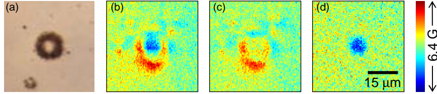
Figure 3.4: Image of an optimally doped YBCO ring obscured by electric charges, taken with a 2\ \mu\text{m} ungated Hall probe. The ring was cooled to T = 70\ \text{K} in zero field. (a) Optical image of a YBCO thin film ring fabricated by Rafael Dinner. (b) Raw V_{xy} image in an applied B -field of 6.5\ \text{G} . (c) Raw V_{xy} image in zero applied B -field. All the features in this zero-field image are due to local electric charges perturbing the Hall probe carrier density. (d) Clean image of the ring shielding the applied 6.5\ \text{G} field obtained by subtracting (c) from (b).
