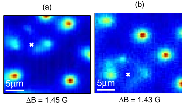
Figure 6.4: Partial vortices prefer certain locations even after annealing the sample at room temperature. (a) T_c = 11.5 K and T = 2.2 K. After six more days at room temperature, (b) T_c = 13.1 K and T = 4.7 K. Note the strikingly similar arrangement of partial vortices surrounding the \times in each image. The \times 's likely mark the same spot on the sample, since a shift between the sample and probe is expected after room temperature thermal cycling. \Delta B is the full scale of the colormap.
