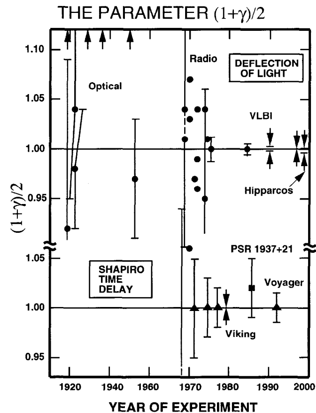
Fig. 5. Measurements of the coefficient (1 + \gamma)/2 from light deflection and time delay measurements. General relativity value is unity. Arrows denote anomalously large values from 1929 and 1936 eclipse expeditions. Shapiro time-delay measurements using Viking spacecraft and VLBI light deflection measurements yielded agreement with GR to 0.1 percent. Hipparcos denotes the optical astrometry satellite.
