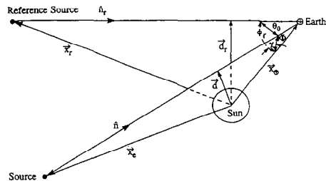
Fig. 4. Geometry of light deflection measurements.
