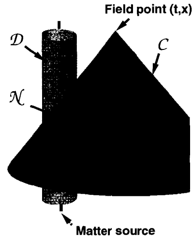
Fig. 7. Past harmonic null cone \mathcal{C} of the field point (t, \mathbf{x}) intersects the near zone \mathcal{D} in the hypersurface \mathcal{N} .
