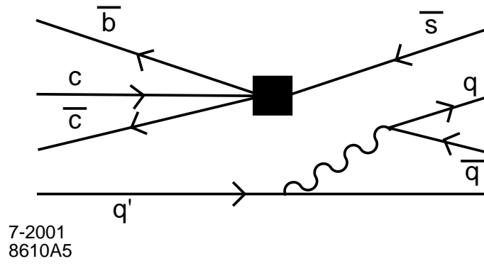
FIG. 5. Hard scattering diagram mediated by intrinsic charm in the B-meson wave function.
