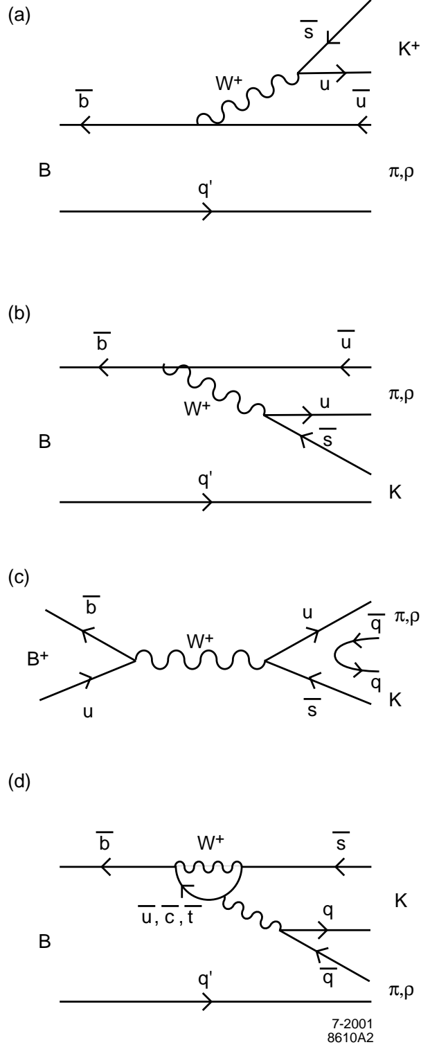
FIG. 2. Schematic illustrations of the full SM contributions to the amplitudes parametrized in Eqs. (2.7- 2.10). Diagram a) contributes to E_1(s, u, u, B, K^+, \pi/\rho) , diagram b) contributes to E_2(u, u, s, B, \pi/\rho, K) , and diagram c) contributes to A_1(s, q, u, B^+, K, \pi/\rho) . Diagram d) contributes to P_1(s, q, B, K, \pi/\rho) and P_1^{GIM}(s, q, B, K, \pi/\rho) .
