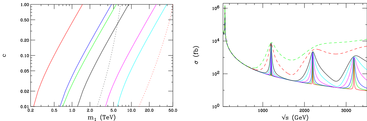
FIG. 4: (Left) Indirect constraints from e^+e^- colliders on the RS model parameter space with c = k/\overline{M}_{Pl} ; the excluded region is to the left of the curves. From left to right the solid curves correspond to bounds from LEP II, a 500 GeV LC with 75 or 500 fb^{-1} luminosity, a TeV machine with 200 fb^{-1} , and a 3 or 5 TeV CLIC with 1 ab^{-1} . The dotted lines are the corresponding LHC (100 fb^{-1} ) and \sqrt{s} = 175 TeV VLHC(200 fb^{-1} ) direct search reaches. (Right) KK graviton excitations in the RS model produced in the process e^+e^- \rightarrow \mu^+\mu^- . From the most narrow to widest resonances the curves are for c in the range 0.01 to 0.2.
