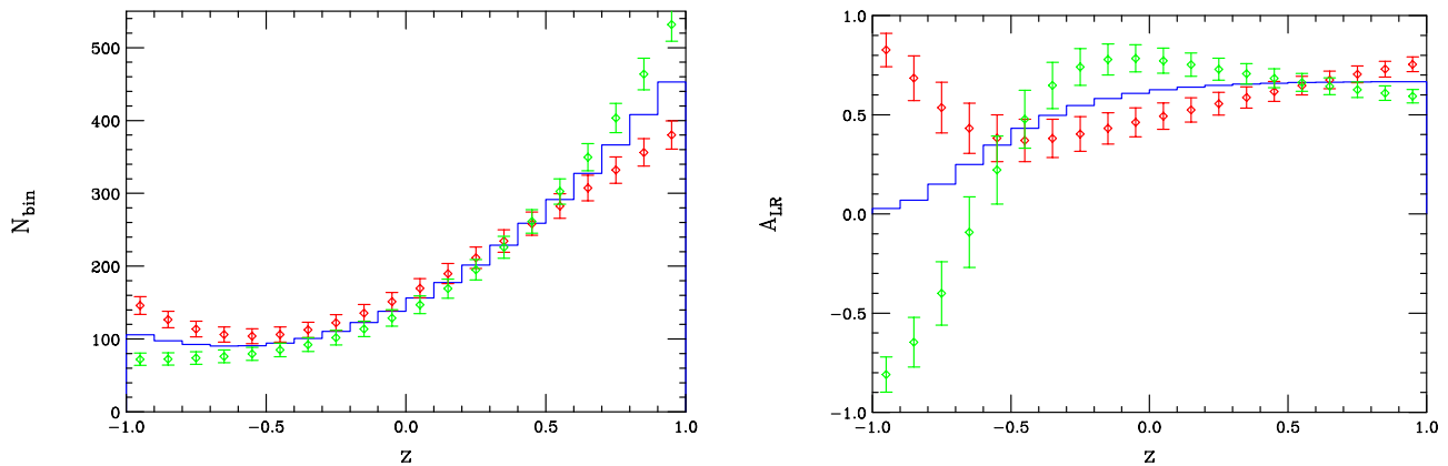
FIG. 1: Deviations in the cross section for \mu -pairs(left) and A_{LR} for b -quarks(right) at \sqrt{s}=5 TeV for M_s = 15 TeV in the ADD model for an integrated luminosity of 1 ab^{-1} . The SM is represented by the histogram while the red and green data points show the ADD predictions with \lambda = \pm 1 . In both plots z = \cos \theta .
