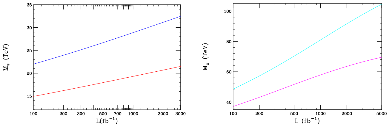
FIG. 2: (Left) Search reach for the ADD model scale M_s at CLIC as a function of the integrated luminosity from the set of processes e^+e^- \rightarrow f\bar{f} assuming \sqrt{s} = 3 (red) or 5(blue) TeV. Here f = \mu, \tau, b, c, t , etc. (Right) Corresponding reach for the compactification scale of the KK gauge bosons in the case of one extra dimension and all fermions localized at the same orbifold fixed point.
