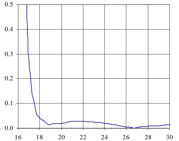
Figure 4: Measured load reflection coefficient magnitude spectra. These values were used to compute the wake.
