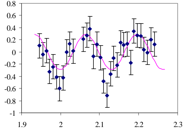
Figure 7: Close-up view of the measured wakefield around 2.1 ns in units of V/(pC \cdot mm) against time in units of ns. A 2.9 V/(pC \cdot mm) 7.6 GHz wake is superimposed on the data.
