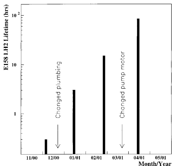
FIGURE 5. LH 2 Lifetime as a Function of the Date of the Experiment
