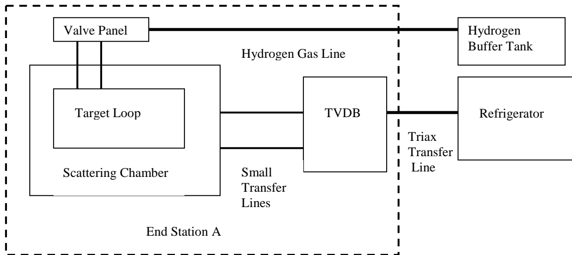
FIGURE 1. Block Diagram of the E158 Cryogenic System
