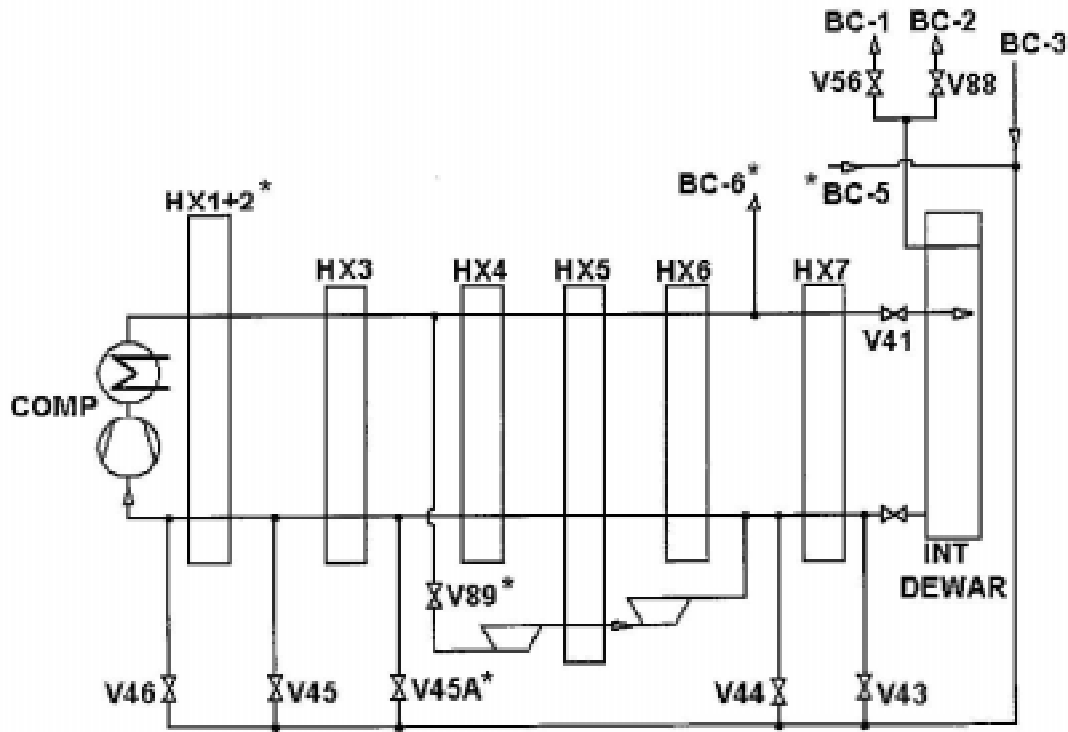
FIGURE 4. Schematic of Upgraded CTI 4000 Refrigerator. * Denotes New Components
