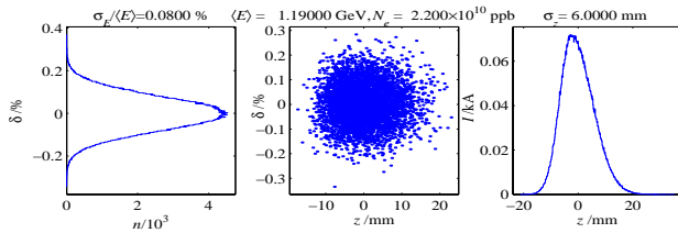
Figure 2. Damping ring longitudinal phase space at 1.19 GeV used for input to tracking studies.
