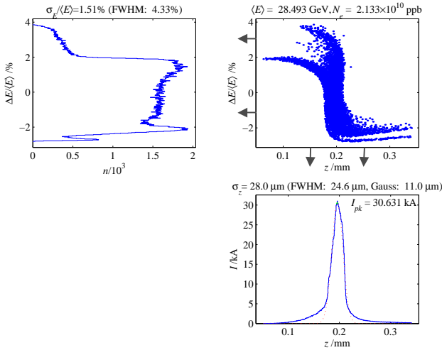
Figure 3. Longitudinal phase space (upper right) at 28.5 GeV after FFTB with distributions (left & bottom). Bunch population is 2.1 \times 10^{10} , energy spread is 1.5% rms, and bunch length is 25- \mu m FWHM with 11- \mu m rms gaussian fit overlaid in red.
