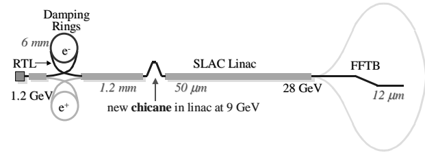
Figure 1. Layout of SLAC linac with 30-kA compression.
