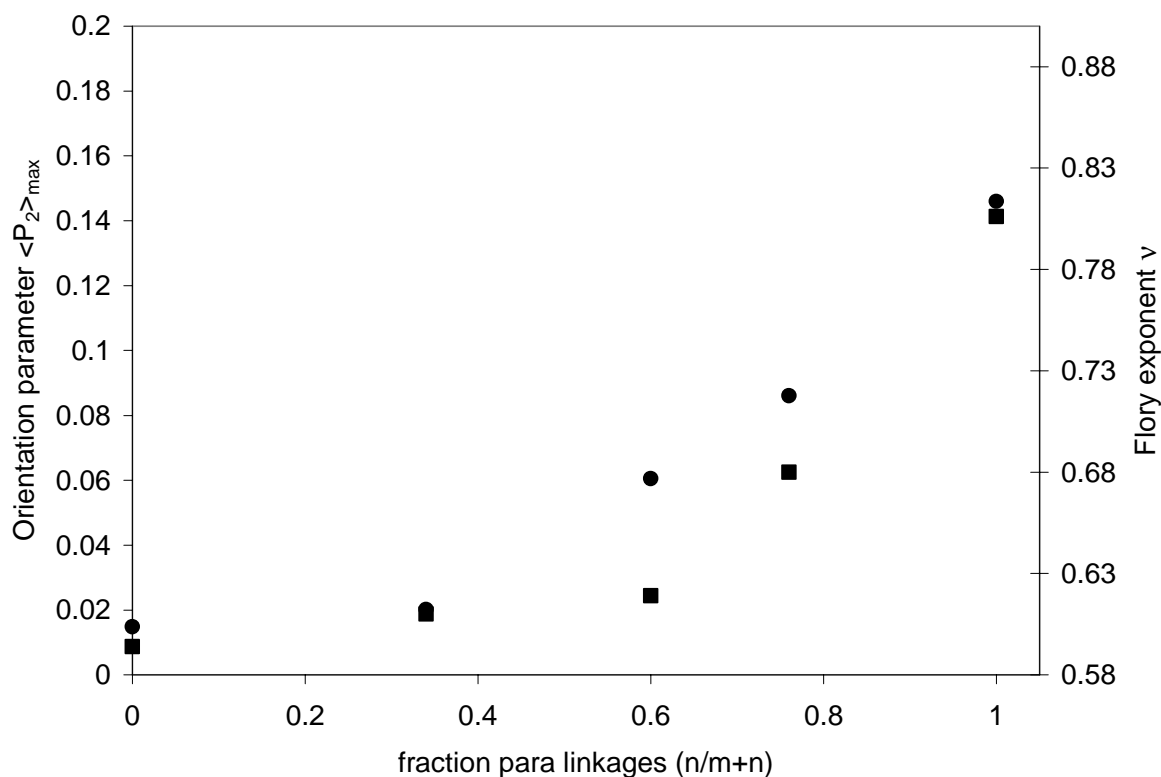
Figure 5a: Maximum orientation (●) observed in azimuthal profiles of SAXS patterns from strained PPyPEH + /PS-co-SS - ionomer blends and Flory exponent (■) from SAXS experiments on PPyPE polymers in dilute solution as a function of the mole fraction of para linkages at the pyridine moiety of the PPyPE molecules.
