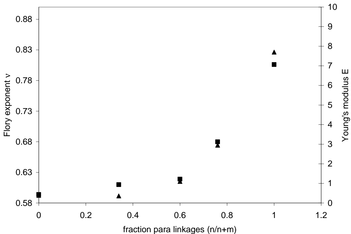
Figure 5b: Flory exponent (■) from SAXS experiments on PPyPE polymers in dilute solution and Young's modulus (▲) of the bulk material from PPyPEH + /PS-co-SS - ionomer blends as a function of the number of para linkages at the pyridine moiety of the PPyPE molecules.
