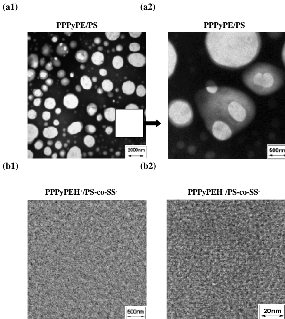
Figure 1: Transmission electron micrographs bright field image of a blend of para-linked poly(pyridyl/phenyl-ethynylene) (PPPyPe) with polystyrene (a1/2) and of the acid-base ionomer blend PPPyPEH + /PS-co-SS - (b1/2) with sulfonated (11mol-% sulfonation) polystyrene (PS-co-SSH); weight fraction PPPyPE 27% in both cases, i.e. stoichiometry of acid/base groups in the ionomer blend; magnification: (a1): 900x; (a2): portion of (a1), 4x; (b1): 9000x; (b2): 125000x
