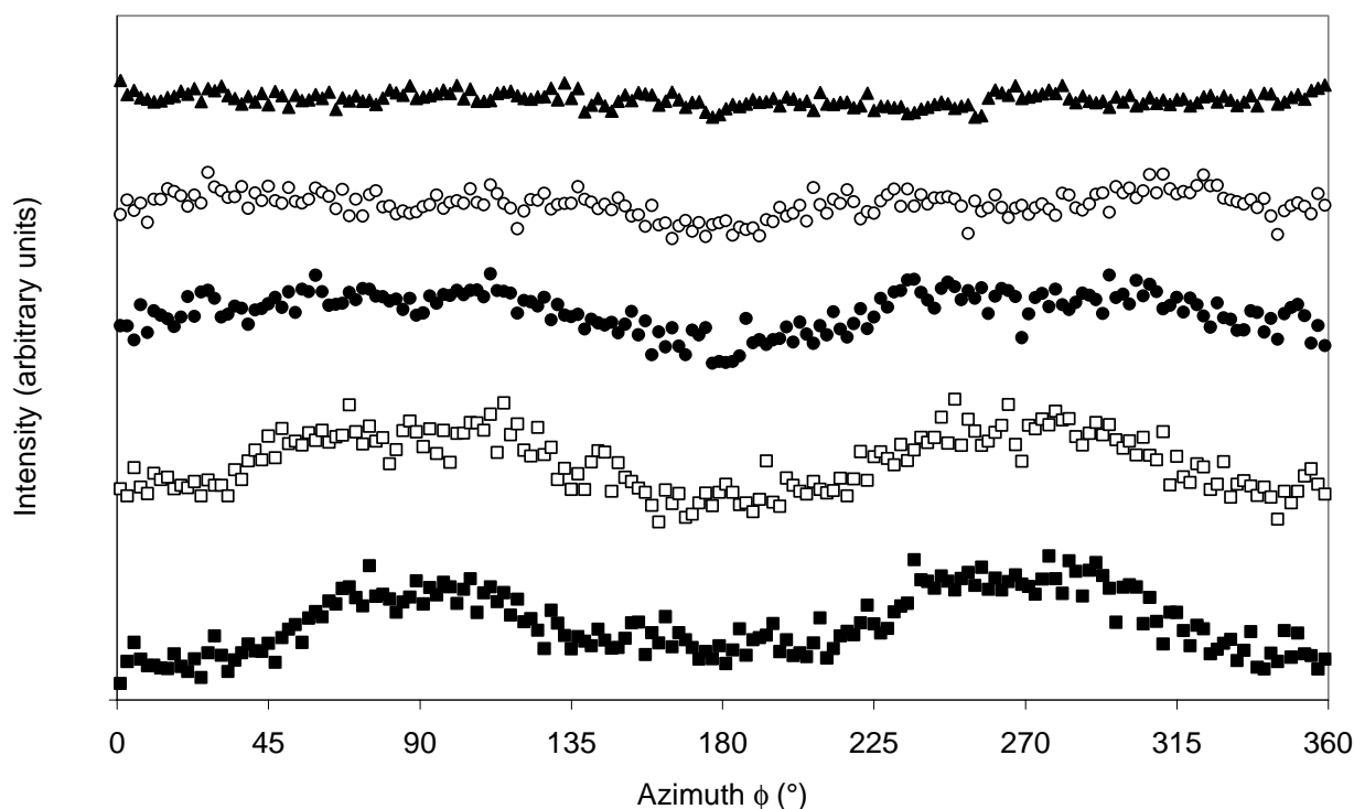
Figure 2: Profiles of intensity against azimuthal angle extracted from SAXS patterns for a poly(pyridyl/phenyl-ethynylene) ionomer blend sample containing only para linkages at the pyridine moiety (PPyPEH + /PS-co-SS - ) strained to 300% extension for various q ranges ( \text{\AA}^{-1} ): 0.103 < q < 0.110 (■); 0.0809 < q < 0.0882 (□); 0.0588 < q < 0.0662 (●); 0.0368 < q < 0.0441 (○); 0.0147 < q < 0.0221 (▲). Intensities are in arbitrary units and not comparable from one profile to another: the profiles are displaced along the ordinate for clarity.
