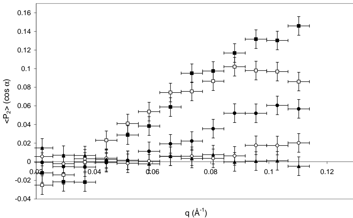
Figure 3: Orientation parameter as a function of scattering vector for five poly(pyridyl/phenyl-ethynylene) ionomer blend samples of varying compositions: PPPyPEH + / PS-co-SS - (■); PCPyPE24H + / PS-co-SS - (□); PCPyPE40H + / PS-co-SS - (●); PCPyPE66H + / PS-co-SS - (○); PMPyPEH + / PS-co-SS - (▲). All samples were strained to 300% extension, except the PMPyPEH + /PS-co-SS - sample (lowest trace) that has been strained to 500%.
