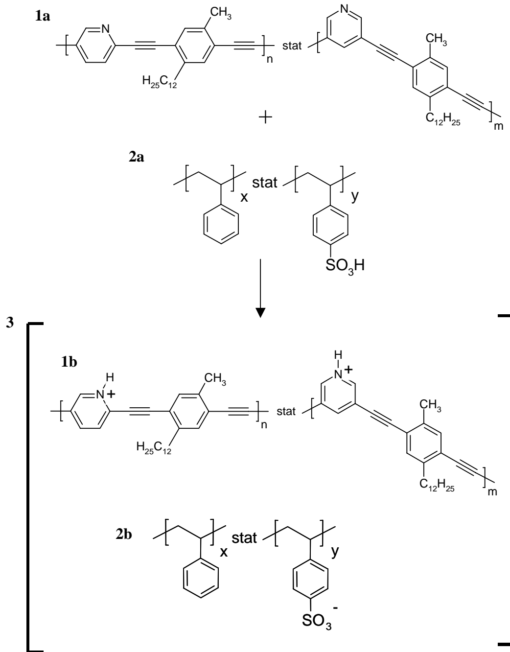
Scheme 1: Chemical structures of the blend components poly(arylethynylene) (PPyPE) rod ( 1a ) and sulfonated polystyrene coil ( 2a ; y/(x+y)=0.11 ) employed in the formation of the acid/base ionomer blends 3 (stoichiometry of pyridyl and sulfonic acid groups) composed of rod polycation ( 1b ) and the coil polyanion ( 2b ).
