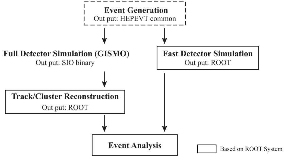
Figure 1: The LCD Simulation/Event analysis flow. Boxed processes are based on the ROOT system. Several event generators are also ROOT-based.
