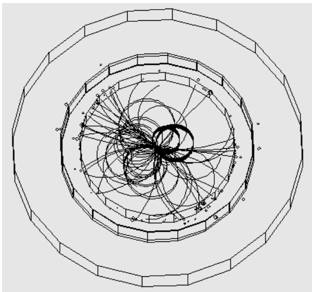
Figure 2: An event display of a simulated 500 GeV e^+e^- \rightarrow t\bar{t} event. Here the Fast simulator assuming the Large detector parameters is used.
