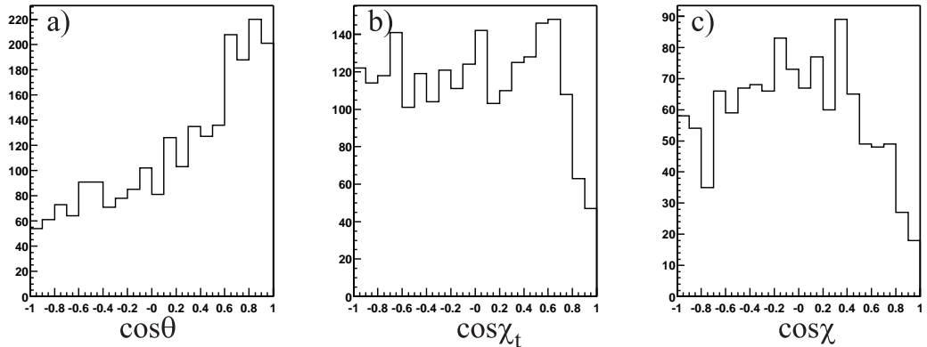
Figure 1: The angular distributions of a) \cos\theta , b) \cos\chi_t and c) \cos\chi for the reconstructed t\bar{t} candidates. The definitions of the \chi_t and \chi are in the text.
