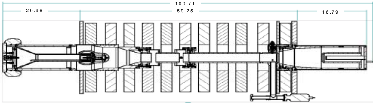
Fig. 4. Cross section of ABK beamstick with magnet coils
