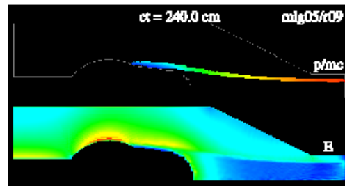
Fig. 2. ISIS Simulation of the MIG
