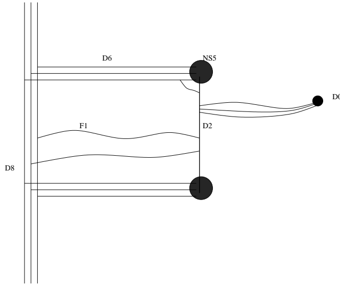
Fig. 4: Long 8-2 strings want to move to the boundary, turn into 6-2 strings and become light. This provides the current which flows into the 1+1 theory on the boundary of the Chern-Simons theory making it anomalous. A D0-brane outside the D2-brane has k strings ending on it. The D0-brane behaves like a soliton with electric charge k and magnetic flux 1. The string ends on the D2-brane behave like anyons of electric charge 1 and magnetic flux \frac{1}{k} .
