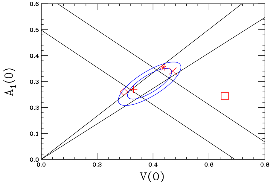
Figure 1: Constraints on the semileptonic form-factors V(0) and A_1(0) from B \rightarrow K^*\gamma data plus HQSS (thicker band) together with the relation from the LEL (cone). The ellipses correspond to 68% and 90% confidence level intervals. Central values of model predictions are also shown and correspond to BSW [12] (vertical cross), ISGW2 [13] (diamond), MS [14] (star), LCSR [15] (diagonal cross) and LW [16] (square), respectively.
