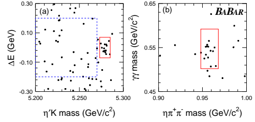
Figure 1: Kinematics of B^+ \rightarrow \eta' K^+ .
