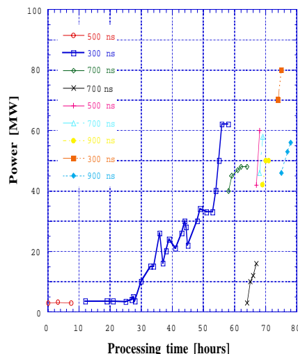
Fig. 2: Processing history for the small type window at KEK
