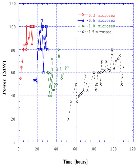
Fig.3: Processing history for the small type window at SLAC
