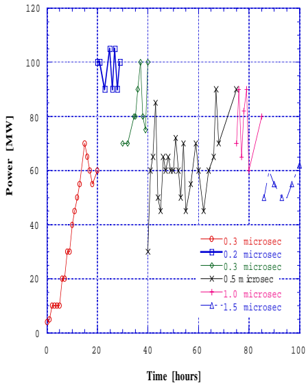
Fig.4: Processing history for the large type window
