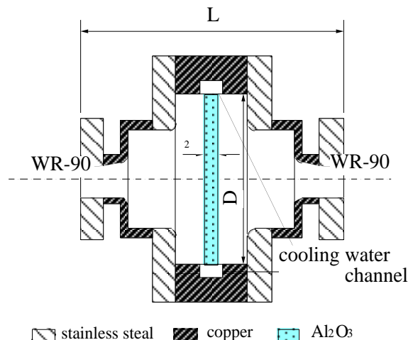
Fig.1: Schematic cross-section of the mixed mode RF window. Length (L) is 85 mm for small size (D=53mm) and 115mm for large size (D=63 mm)
