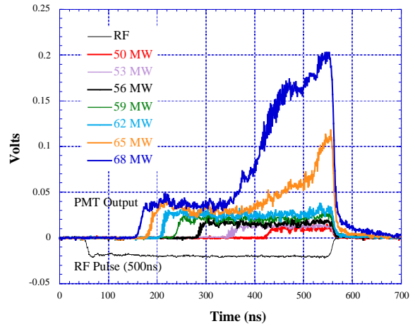
Fig. 5: Observed PMT signals at high power test of large size window.
