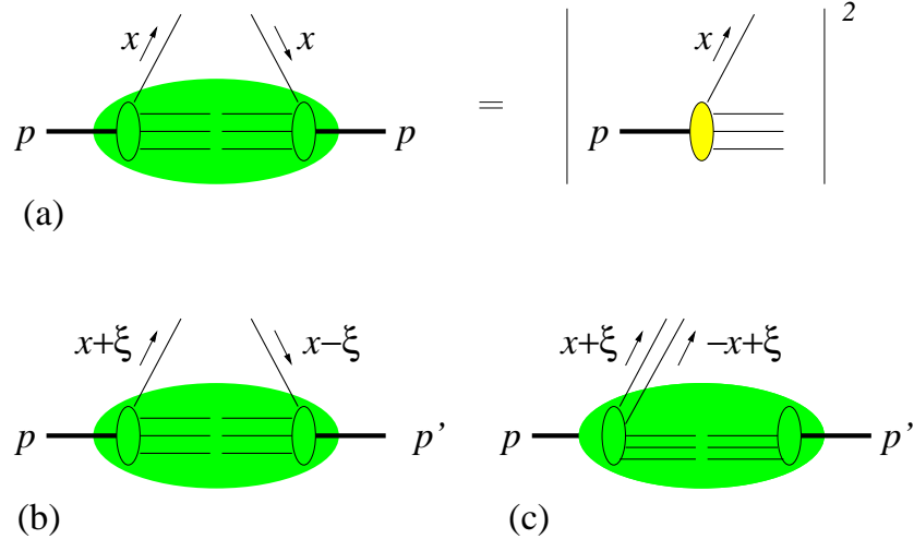
Figure 2: (a) Usual parton distribution, representing the probability to find a parton with momentum fraction x in the nucleon. All configurations of the spectator partons are summed over. (b) SPD in the region where it represents the emission of a parton with momentum fraction x + \xi and its reabsorption with momentum fraction x - \xi . (c) SPD in the region where it represents the emission of a parton pair. Here x + \xi > 0 and x - \xi < 0 .
