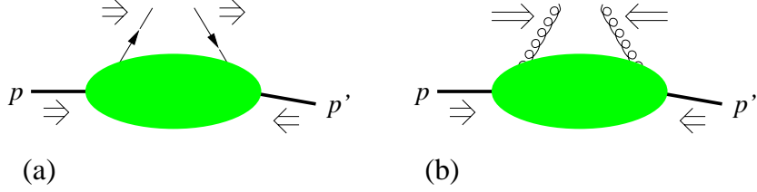
Figure 3: (a) SPD which flips the helicity of the proton but not of the quark. A unit of orbital angular momentum must be transferred. (b) SPD which flips the gluon helicity. Again there must be transfer of orbital angular momentum.
