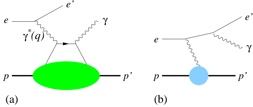
Figure 1: (a) A Born level diagram for DVCS. The blob represents a skewed quark distribution. (b) A diagram for the Bethe-Heitler process. The blob here stands for an elastic proton form factor.
