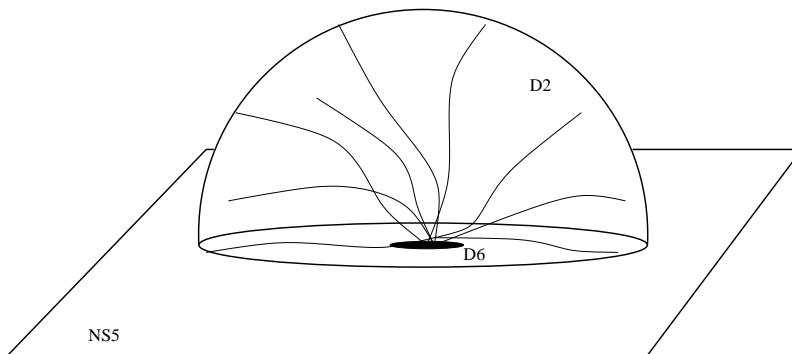
Figure 4: Here we see a hemi-spherical D2-brane ending on an NS 5-brane. K D6-branes are embedded in the NS 5-brane. K strings stretch to the D2-brane.
