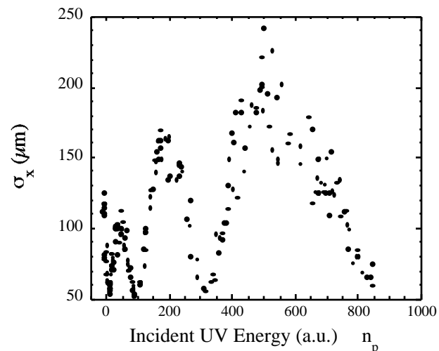
Figure 3: Beam spot size measured at the downstream OTR location as a function of the relative uv laser pulse energy. The plasma density is proportional to the uv energy.
