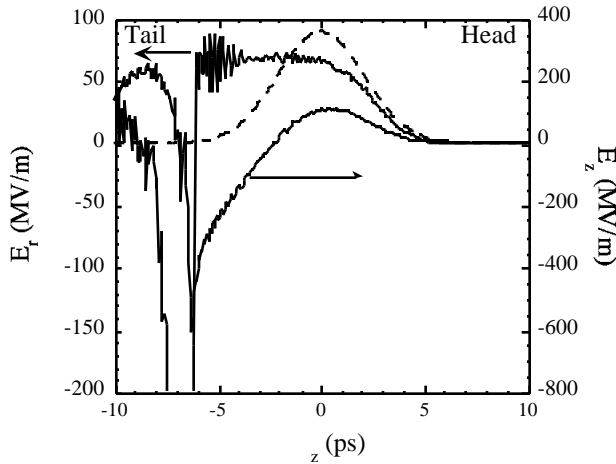
Figure 1: Transverse ( E_r , thin line, left hand side scale) and longitudinal ( E_z , thick line, right hand side scale) wake fields excited by the beam (shown by the dotted line) with parameters given in Table 1 in a plasma with n_p = 1.5 \cdot 10^{14} \text{ cm}^{-3} .
