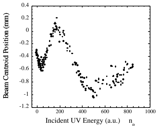
Figure 4: Beam centroid position measured by a beam position monitor located 2.5 m downstream from the plasma exit. This data was acquired at the same time as the beam spot size data shown on Fig. 3.
