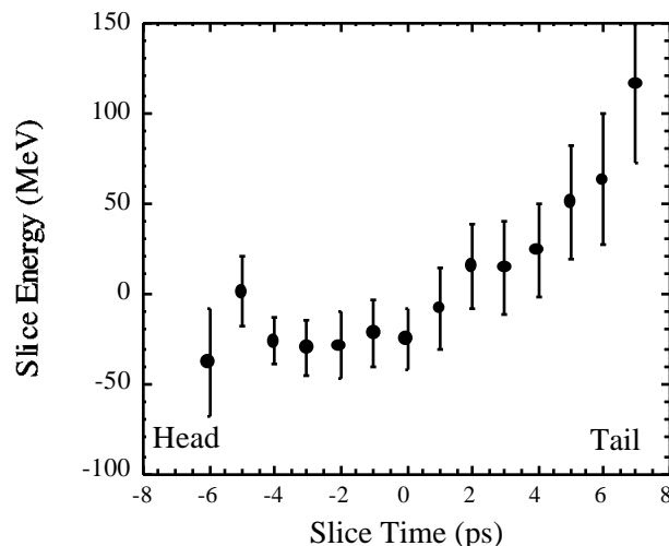
Figure 5: Result of the slice analysis showing the average energy of 1 ps slices obtained from 23 individual images. The core ( -2 ps) of the beam loses energy, where as the slices in the tail gain energy (see Fig. 2).
