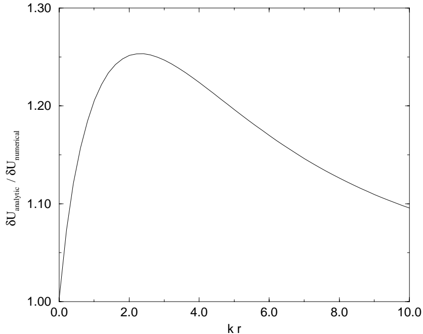
FIG. 1. A comparison of (8) with (5) is given. The Newtonian potential is given by -(G_N m_{source}/r)(1 + \delta U_X) where \delta U_{analytic} is given by Eq. (5) and \delta U_{numerical} is given by Eq. (8).
