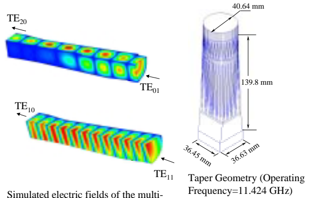
Simulated electric fields of the multimoded circular to rectangular taper
