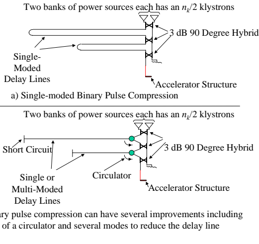
Fig. 1 Binary Pulse Compression system
